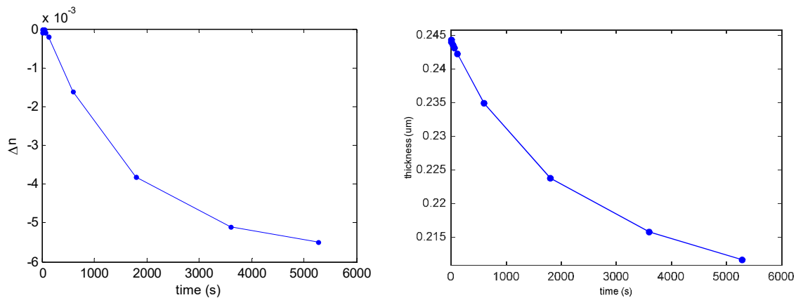
Figure 7. On the left: refractive index modulation as function of time at room temperature in the dark; on the right: film thickness evolution as function of the elapsed time.
