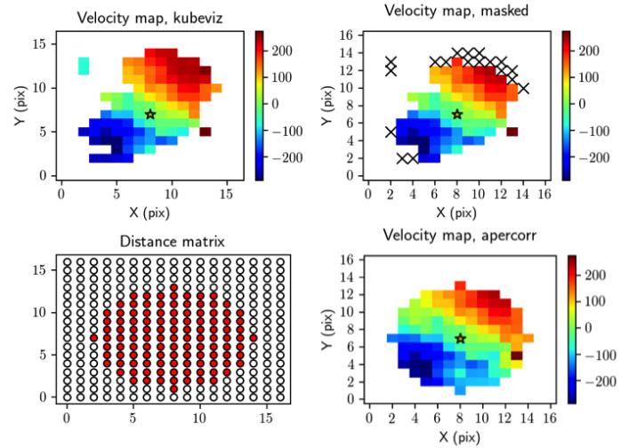
Fig. 9. Summary of procedure followed to estimate the H\alpha flux within the 1''/2 radius aperture, for a typical case of a galaxy with a rotation curve. Top-left panel: velocity map from KUBEVIZ. The star at the centre of the image represents the pixel position from which the aperture is estimated. Bottom-left panel: distance matrix that defines the six-pixel radius corresponding to the aperture. Top-right panel: shows which spaxels from the original map are discarded because they fall outside the aperture. Bottom-right panel: corrected velocity field obtained following the procedure described in the main text for assigning a peculiar velocity to the spaxels flagged as bad in KUBEVIZ.
