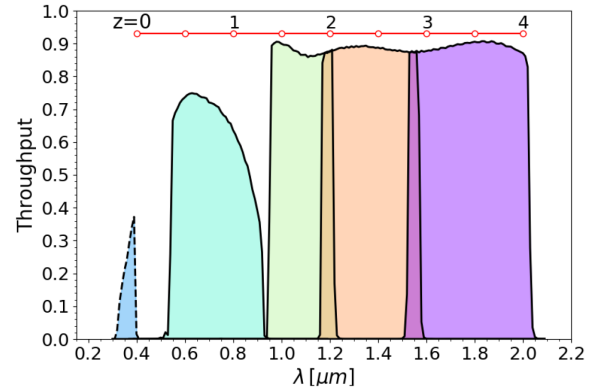
Figure 1. Throughput of the four main Euclid filters (coloured regions and solid black lines). From the left- to right-hand side, these are the VIS filter, and the NISP/ Y , NISP/ J , and NISP/ H filters. We also include the throughput of the CFIS/ u -band filter (blue region, dashed black line). The red dots indicate the observed wavelength of the 4000-Å break at different redshifts.
