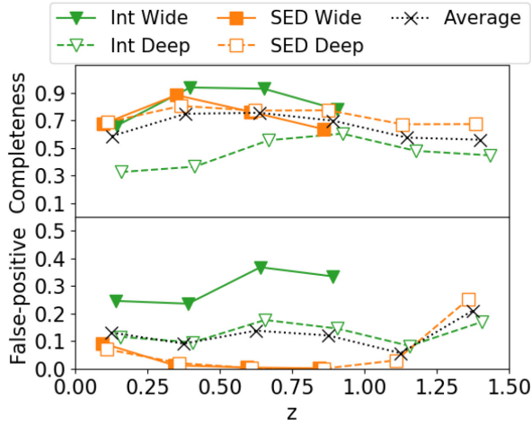
Figure 9. Evolution of the completeness and FP fraction with the redshift (left-hand panel) and with the observed VIS magnitude (right-hand panel). Quiescent galaxies are derived considering the best line separation in the (u - VIS) versus (VIS - J) plane, as described in equation (2). The fractions correspond to the mock observations derived from the best SED template (orange squares) and from interpolating the COSMOS2015 observations (green triangles), considering the observational depth expected for the Euclid Wide Survey (coloured symbols) and the Euclid Deep Survey (empty symbols). Black crosses are the average values among the four considered data sets. Coloured data points are slightly shifted horizontally for clarity, while black crosses mark the centre of each bin. The grey dotted vertical lines on the right-hand panel show the VIS magnitude corresponding to different S/N cut in the Euclid Wide Survey.
