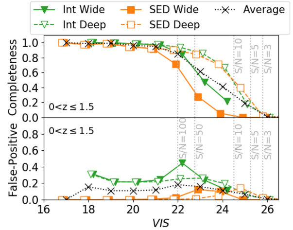
Figure 9. Evolution of the completeness and FP fraction with the redshift (left-hand panel) and with the observed VIS magnitude (right-hand panel). Quiescent galaxies are derived considering the best line separation in the (u - VIS) versus (VIS - J) plane, as described in equation (2). The fractions correspond to the mock observations derived from the best SED template (orange squares) and from interpolating the COSMOS2015 observations (green triangles), considering the observational depth expected for the Euclid Wide Survey (coloured symbols) and the Euclid Deep Survey (empty symbols). Black crosses are the average values among the four considered data sets. Coloured data points are slightly shifted horizontally for clarity, while black crosses mark the centre of each bin. The grey dotted vertical lines on the right-hand panel show the VIS magnitude corresponding to different S/N cut in the Euclid Wide Survey.
