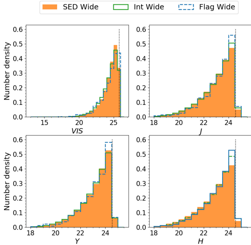
Figure A2. Distribution of magnitudes in the VIS (top left-hand panel), J (top right-hand panel), Y (bottom left-hand panel), and H (bottom right-hand panel) bands for galaxies in the three different data sets considered in this work: SED Wide (filled orange histograms), Int Wide (green solid lines), and Flag Wide (blue dashed lines). The vertical dotted lines indicate the magnitude corresponding to a S/N = 3 for each filter.
