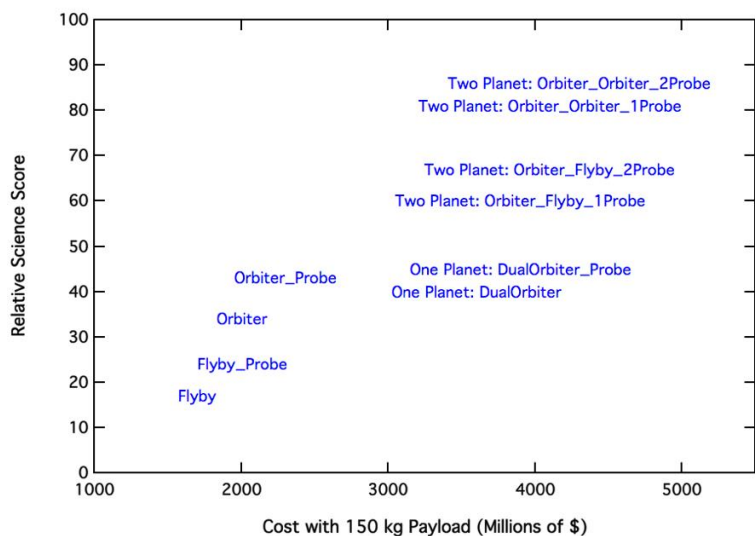
Fig. 6 Relative science value versus approximate cost for a subset of missions considered. Costs should be read from the center of the mission label (e.g. the “i” in Orbiter), but note the factors discussed in the text that can alter these numbers. For comparison purposes, all spacecraft plotted have a 150 kg science payload. Smaller payloads will reduce the science ranking, but will also reduce single-spacecraft costs by up to $600M and dual-spacecraft costs by up to $1100M. Single-planet missions are costed for Uranus; Neptune costs will be about $300M higher. Architectures are divided into three groups by their science value: flybys, single-planet orbiters, and dual-planet missions. Note that the recommended mission, an orbiter with probe, occupies a “plateau” in science value vs. cost, and is the least expensive option that achieves that level of science. See the IG Study for additional discussion. This figure is an updated version of Fig. 3-17 of the IG Study
