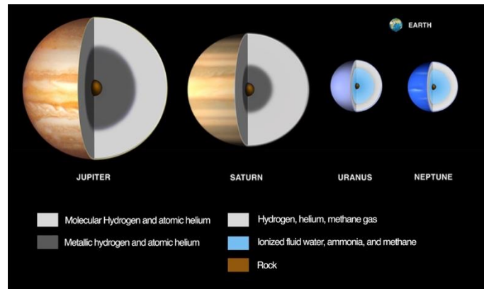
Fig. 1 Illustration of compositional and structural differences among the giant planets and their relative sizes. Earth is shown for comparison. Jupiter and Saturn are primarily made of hydrogen and helium, the terrestrial planets are almost pure rock, while Uranus and Neptune are thought to be largely supercritical water
