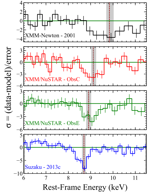
Figure 1. Residuals to the power-law continuum fitted between 2 and 10 keV band from four selected observations of PDS 456 decreasing in X-ray luminosity. This shows how the centroid energy of the Fe K absorption profile generally decreases in energy with decreasing luminosity from top to bottom. The vertical dotted lines and the grey shadowed areas indicate the position of the centroid and the 90 per cent uncertainty (see Table 2).
