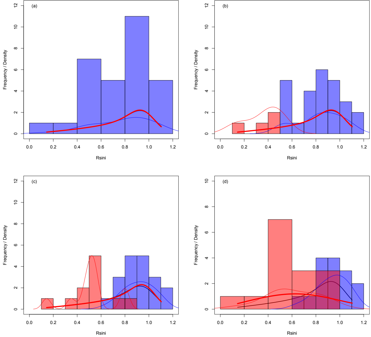
Fig. A.1. Illustrative tests in recovering \mathcal{R} from a synthetic \{R \sin i\} set with censoring. The simulations reproduce n = 30 slow-rotator sequence stars in the Pleiades with M \sim 1 M_{\odot} and R \sim 1 R_{\odot} at varying censoring levels: (v \sin i)_{\text{lim}} = 0 (panel a )); 6 (panel b )); 9 (panel c )); 10 (panel d )) \text{km s}^{-1} . Blue and red histograms are used for censored and not-censored data. The kernel density estimate is shown as a thin blue line for not-censored data and as a red thin line for censored data, the function \phi corresponding to the given synthetic distribution parameters is plotted as a thick black line and that corresponding to the reconstructed parameter as a thick red line. Histograms are representations of frequency.
