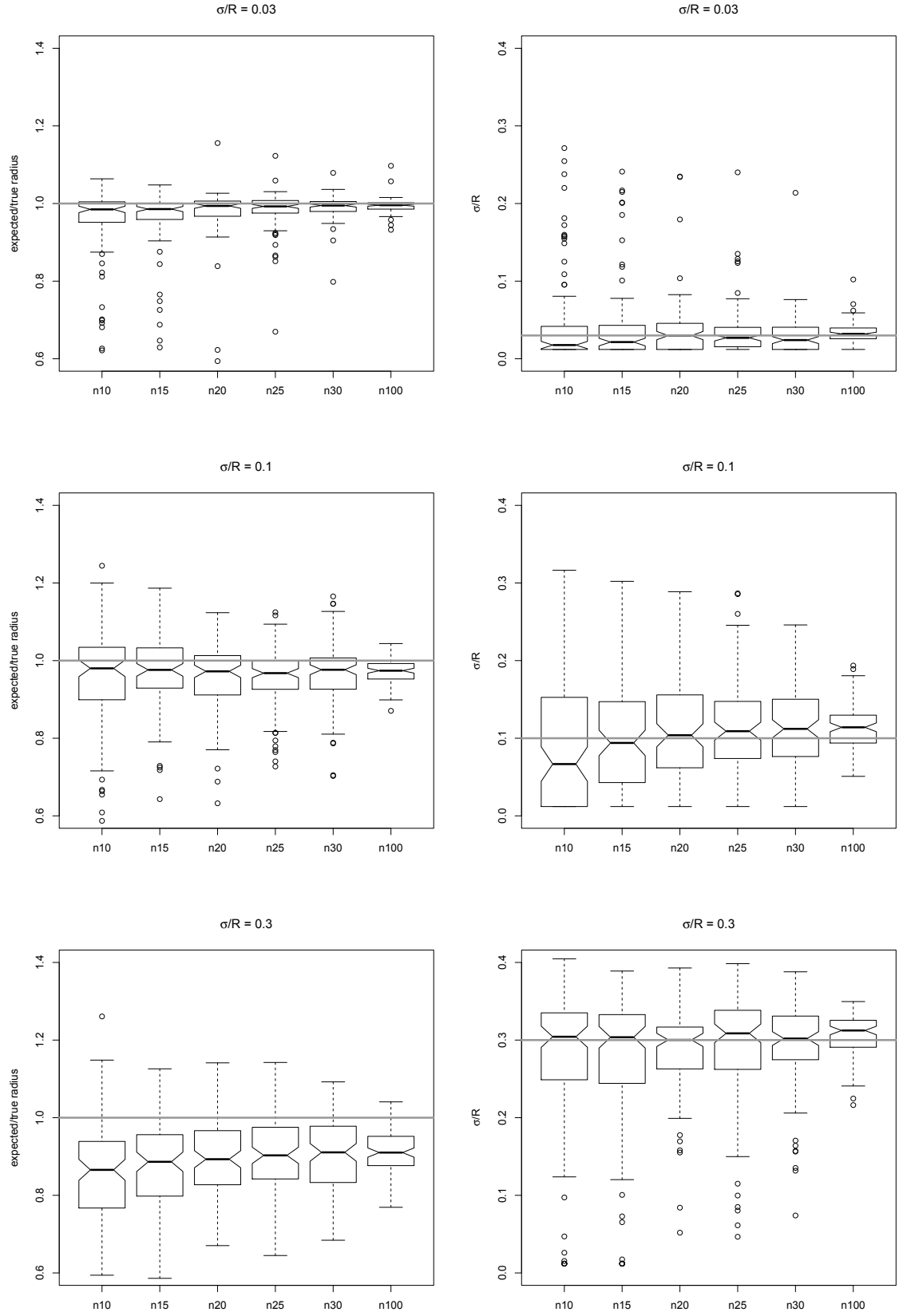
Fig. A.3. Box-and-whisker plots for the reconstructed \mathcal{R} and \sigma from 100 random realisations of the R \sin i distribution with censoring and truncation at different \sigma/\mathcal{R} values and different number of measurements per bin.
