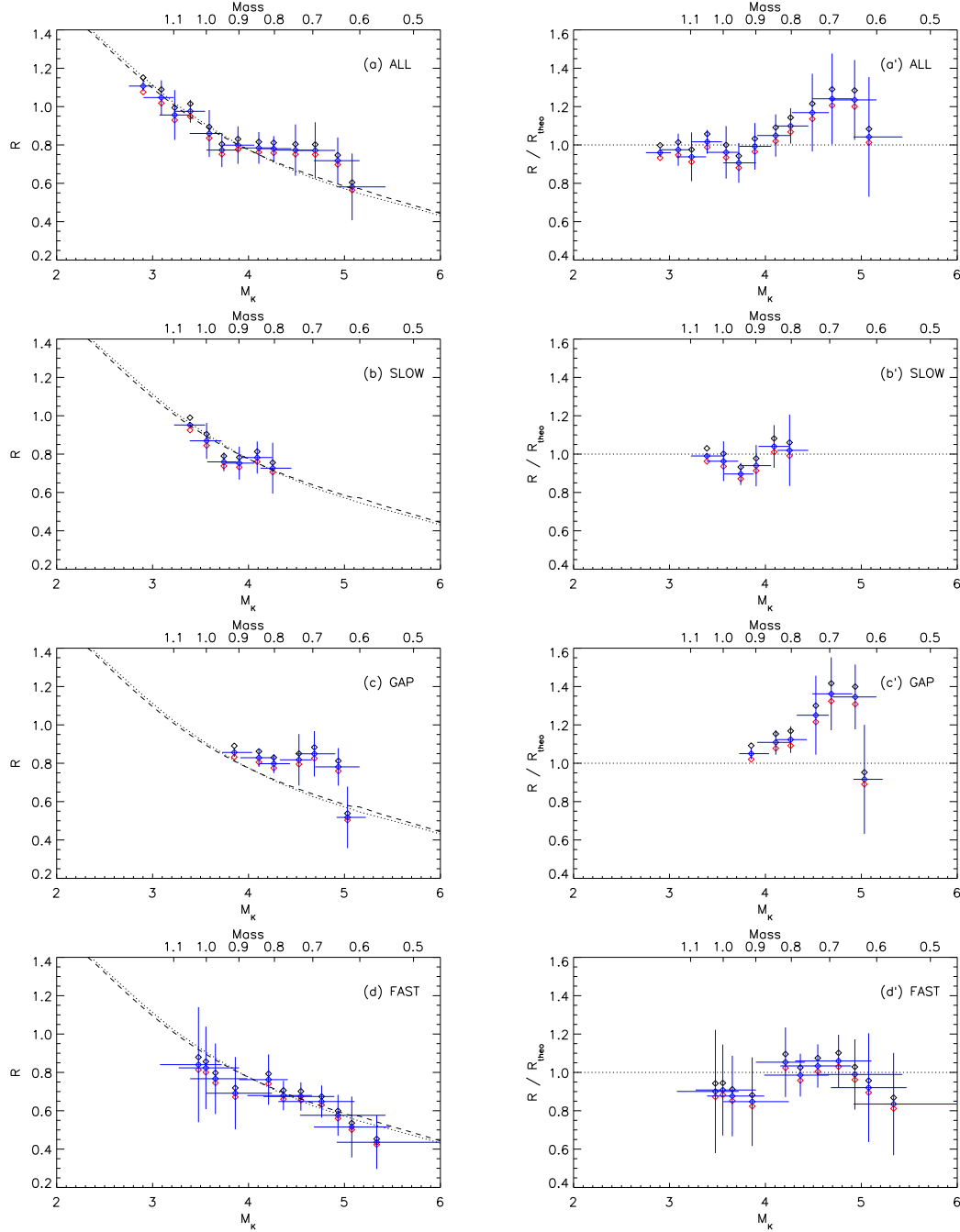
Fig. 3. Comparison of the expected radius \mathcal{R} with the models of Baraffe et al. (2015; dotted line) and Spada et al. (2013; dashed line). \mathcal{R} is reported as a function of the average M_K in each bin. The three values of \mathcal{R} correspond to our best estimate of the SDR (blue diamond) and the estimated upper and lower SDR limits (black and red diamonds). The horizontal bars encompass the M_K range in each bin. The vertical bars represent the standard deviation \sigma for each bin centred on our best estimate of the SDR. Right panels show the ratio with the Baraffe et al. (2015) model. Panels a) and a') are obtained using all data, panels b) and b') for the slow-rotator sequence, panels c) and c') for stars with periods between fast and slow rotators, panels d) and d') for fast rotators only ( P < 2 d). Bins are \Delta M \approx 0.1 M_\odot wide except for the fast rotators set, for which \Delta M \approx 0.2 M_\odot to ensure that at least \approx 10 stars fall in each bin.
