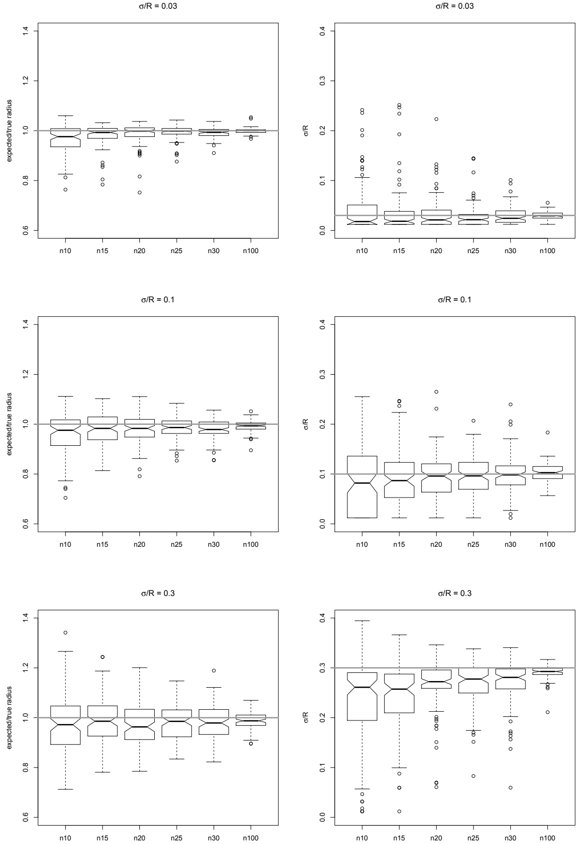
Fig. A.2. Box-and-whisker plots for the reconstructed \mathcal{R} and \sigma from 100 random realisations of the R \sin i distribution with no censoring and no truncation at different \sigma/R values and different number of measurements per bin.
