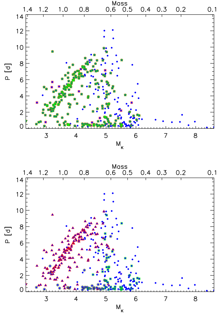
Fig. 1. Hartman et al. (2010) P dataset of the Pleiades (blue filled circles). Upper panel: open red squares outline targets for which v \sin i is available and green stars those considered in this work. Lower panel: open red triangles indicate v \sin i from Queloz et al. (1998), green squares the values adopted from Terndrup et al. (2000), plum pentagons those from Stauffer & Hartmann (1987), and olive hexagons those from Soderblom et al. (1993). See text for details.
