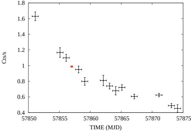
Fig. 6. Flux evolution of SXP59.0 during the 2017 outburst, as observed with Swift /XRT. The red symbol corresponds to the epoch and flux (with its uncertainty) of the XMM-Newton observation.
