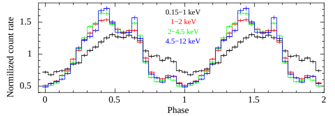
Fig. 3. Pulse profile of SXP59.0 in the energy ranges 0.15–1, 1–2, 2–4.5, and 4.5–12 keV.
