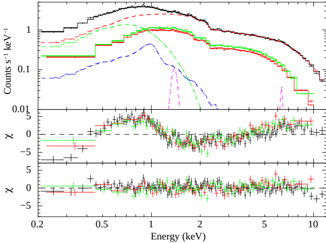
Fig. 4. Time-averaged spectrum of SXP59.0. Black, red, and green symbols respectively represent pn , MOS1, and MOS2 data. Upper panel: superposition of the EPIC spectra with (for the pn spectrum only) the best-fitting model composed of PL+BB+APEC (red, green, and blue dashed lines, respectively) and the Gaussian components (magenta dashed lines). Middle panel: data-model residuals obtained when fitting the spectra with a simple PL model. Lower panel: data-model residuals obtained with the best-fitting model.
