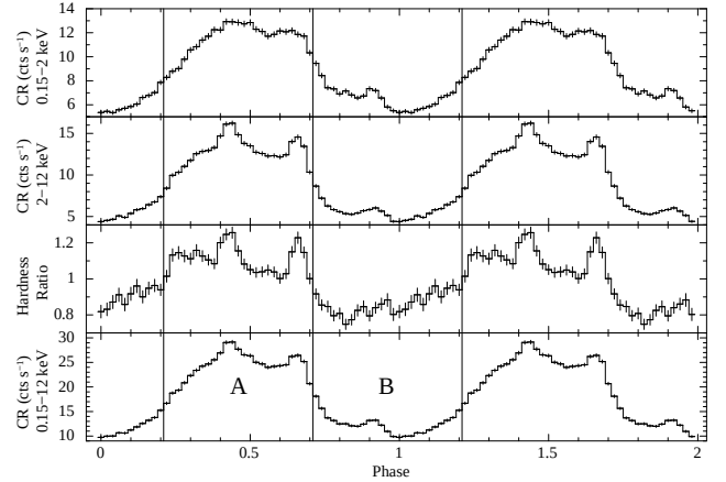
Fig. 2. Light curves of SXP59.0 in the energy ranges 0.15–2, 2–12, and 0.15–12 keV, folded on the period P = 58.949 s. The two phase intervals selected for the phase-resolved spectral analysis (Sect. 6) are delimited by vertical lines.
