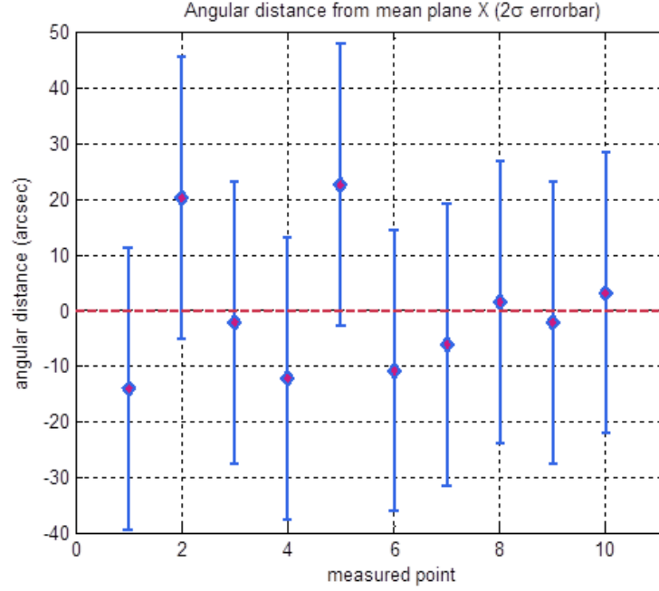
Figure 15: Distribution of measurements evaluated in terms of angular distance from the estimated X non-sensitivity plane. Standard deviation at 2\sigma_0 , std_{hc} = 25.24 arcsec
