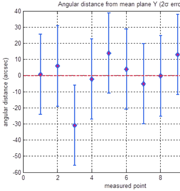
Figure 16: Distribution of measurements evaluated in terms of angular distance from the estimated Y non-sensitivity plane. Standard deviation at 2\sigma_0 , std_{hc} = 24.89 arcsec
