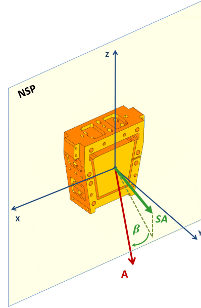
Figure 5: Rotation of the sensor (hence of the sensing axis) by an angle \beta with respect to an applied acceleration ( \vec{A} )
