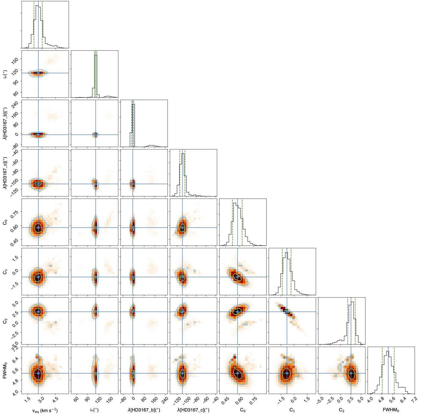
Fig. 12. Correlation diagrams for the PDFs of the RMR model parameters from the joint fit to the HD 3167b and HD 3167c transits (same details as in Fig. 8).
