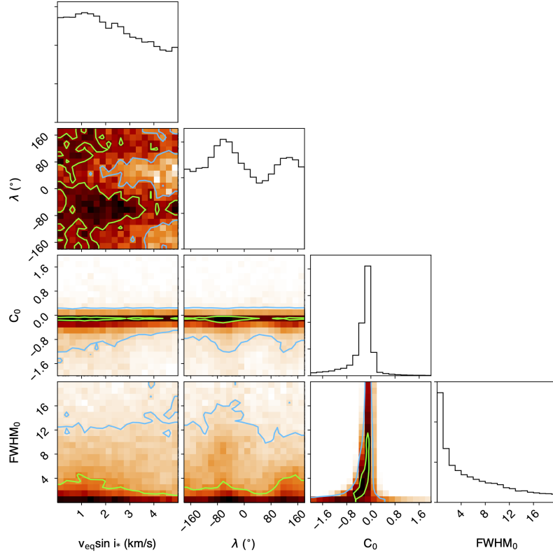
Fig. A.1. Correlation diagrams for the probability distributions of the RMR model parameters, for the fit performed in the blue continuum of the CCF_{intr} .
