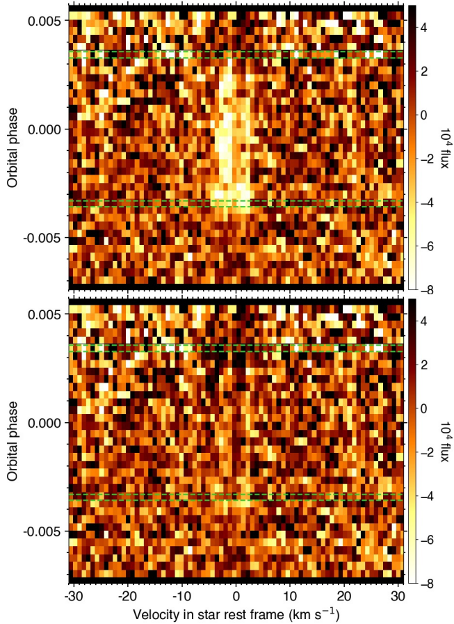
Fig. 9. Maps of the out-of-transit residual \text{CCF}_{\text{loc}} , and of the in-transit residuals between \text{CCF}_{\text{intr}} and their best-fit model (from the joint fit to both transit datasets), during the HD 3167c visit. Transit contacts are shown as green dashed lines. In the top panel , only the continuum of the \text{CCF}_{\text{intr}} model was subtracted to highlight the occulted stellar lines. In the bottom panel , the full line model was subtracted.
