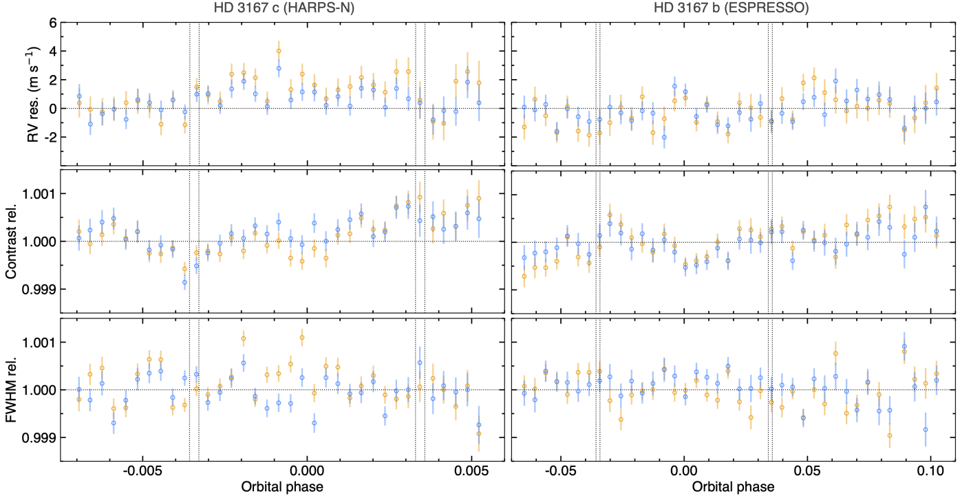
Fig. 1. Time series properties derived from the HARPS-N ( left panel ) and ESPRESSO ( right panel ) CCF DI calculated with the masks previously used by the instruments’ DRS (orange) and with masks built with an improved definition of the line weights and a line selection specific to HD 3167 (blue). Top panels show Keplerian RV residuals. Middle and bottom panels show the contrast and FWHM relative to their out-of-transit mean value, so that they can be compared between the different masks. Vertical dashed lines show the transit contacts of the observed HD 3167 planets.
