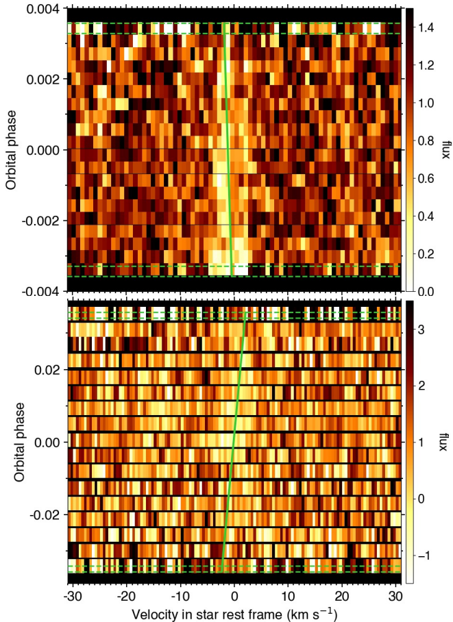
Fig. 3. Maps of the \text{CCF}_{\text{intr}} during the transits of HD 3167 c (HARPS-N, upper panel ) and HD 3167 b (ESPRESSO, lower panel ). Transit contacts are shown as green dashed lines. Values are colored as a function of their normalized flux and plotted as a function of RV in the stellar rest frame (in abscissa) and orbital phase (in ordinate). HD 3167c is large enough that the stellar line can be distinguished in individual exposures, while the small transit depth of HD 3167b makes the line undetectable in most exposures even with the VLT/ESPRESSO data. The green solid lines show the best-fit models for the stellar surface RVs derived with the joint RMR fit to both data sets.
