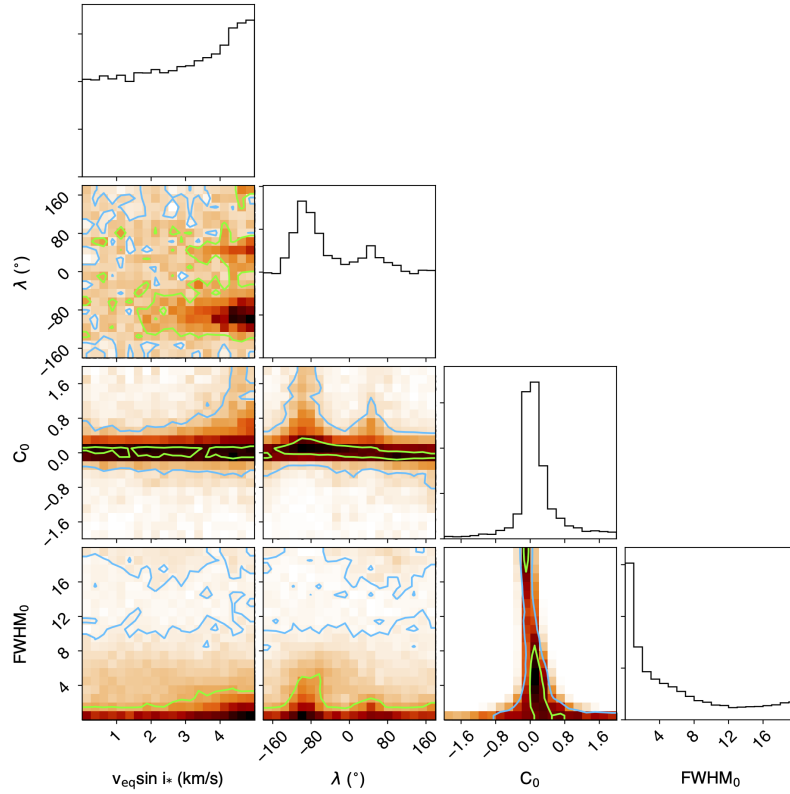
Fig. A.2. Correlation diagrams for the probability distributions of the RMR model parameters, for the fit performed in the red continuum of the CCF_{intr} .
