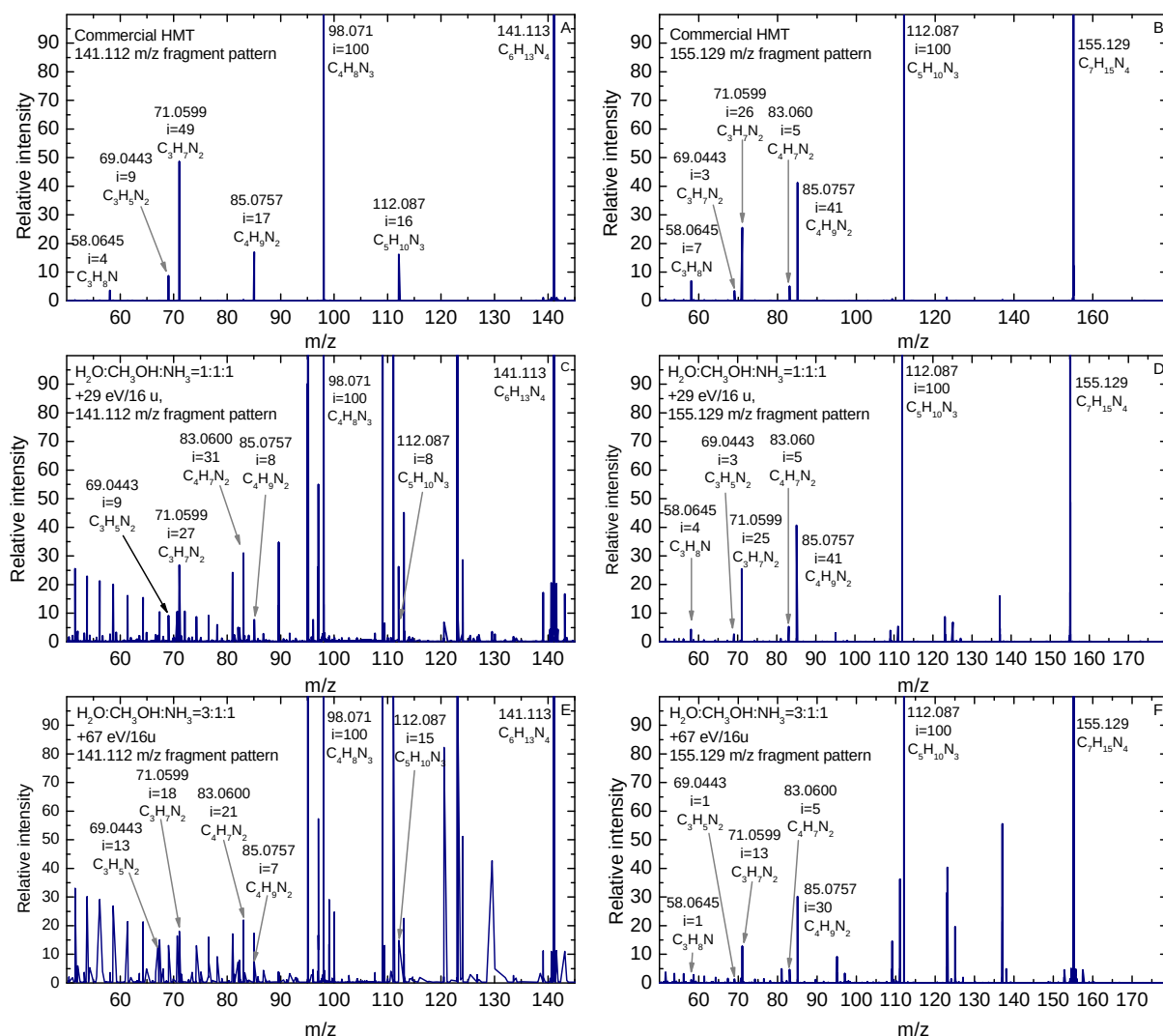
Fig. 9. Fragment pattern of peaks at 141.113 (left panels) and 155.129 m/z (right panels) of: Panels A and B: commercial HMT; panels C and D: 1:1:1 + 29 eV/16 u residue; panels E and F: 3:1:1 + 67 eV/16 u residue. For each fragment, labels indicate the m/z value, the intensity with respect to the most intense fragment, and the stoichiometric formula of the detected molecular ion M+H^+ .
