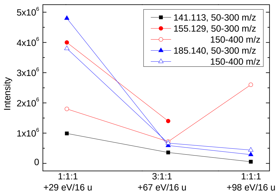
Fig. C.1. Intensity of m/z peaks of molecular ions with the same stoichiometric formulas of \text{HMT}^+ , \text{HMT-CH}_3\text{H}^+ , and \text{HMT-C}_2\text{H}_5\text{OH}^+ .
