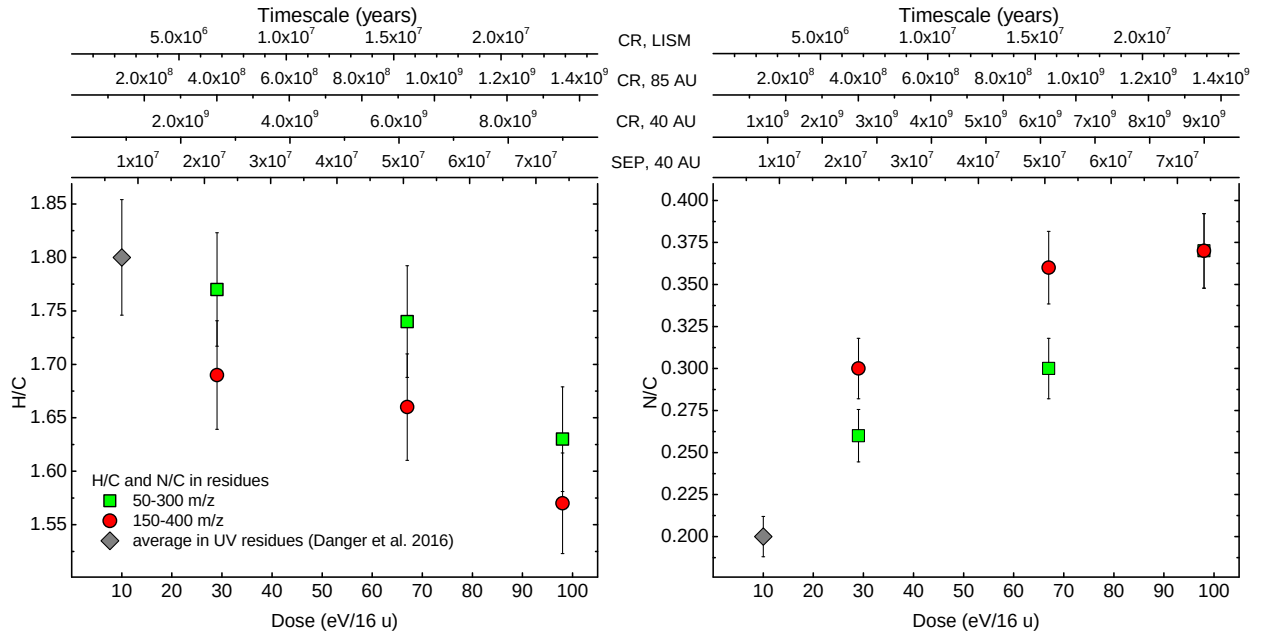
Fig. 4. Ratios of H/C and N/C in organic refractory residues produced after irradiation with 40 keV \text{H}^+ . Grey rhombus give the average elemental ratios of UV residues analysed by means of VHRMS in both positive and negative electron spray ESI modes in the range 50–400 m/z by Danger et al. (2016). The bars refer to the relative standard deviation (RSD) given by Fresneau et al. (2017): 3% for H/C and 6% for N/C values. Top x-axes give the timescale necessary for a frozen surface (50 \mu\text{m} thick) to accumulate the dose given in the bottom x-axes. To calculate timescales, we take into account four cases: bombardment by SEP on a surface located at 40 AU; bombardment by CR for a surface at 40 AU; bombardment by CR on a surface at 85 AU, bombardment by CR on a surface in the Local Interstellar Medium (LISM), which is beyond 100 AU. Timescales do not take into account the time needed for a surface to experience the heating necessary for the production of organic refractory materials.
