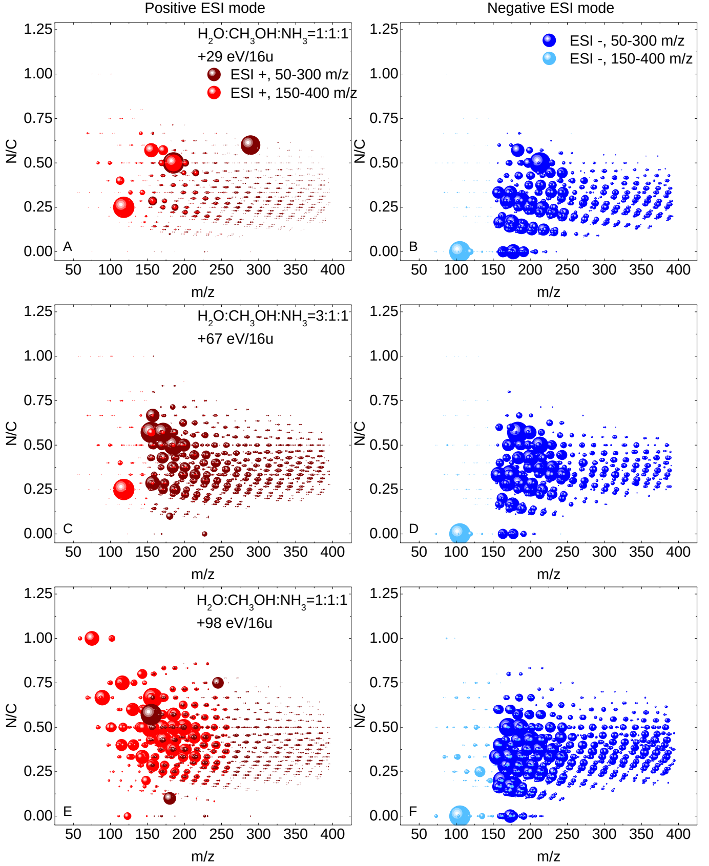
Fig. B.4. Ratios of N/C with respect to the m/z ratio in the range 50–300 and 150–400 m/z in positive ESI mode (left panels) and negative ESI mode (right panels). Panels A and B: 1:1:1 + 29 eV/16 u residue; panels C and D: 3:1:1 + 67 eV/16 u residue; panels E and F: residue of the 1:1:1 + 98 eV/16 u. The size of the dots is given by the normalized intensity.
