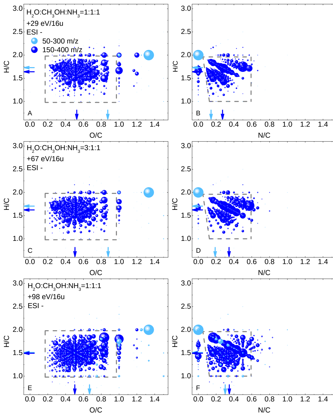
Fig. 7. van Krevelen scatter plots of hydrogen to carbon versus mass oxygen to carbon ( left panels ) and versus nitrogen to carbon ( right panels ) in the three residues analysed in negative ESI mode in the mass ranges 50–300 (light-blue dots) and 150–400 (blue dots). Panels A and B: 1:1:1 + 29 eV/16 u residue; panels C and D: 3:1:1 + 67 eV/16 u residue; panels E and F: 1:1:1 + 98 eV/16 u residue. The size of the dots is given by the normalized intensity. Grey dashed lines delimit the zone of highest density of ions observed in the residues analysed by Danger et al. (2016) . Arrows show the H/C, O/C and N/C weighted averages reported in Table 2 for the range 50–300 m/z (cyan arrows) and 150–400 m/z (blue arrows).
