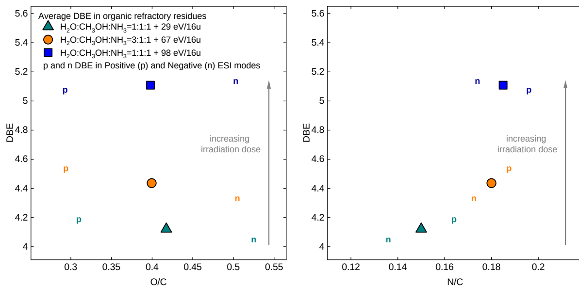
Fig. 8. Double bond equivalent (DBE) versus O/C ( left panel ) and N/C ( right panel ) measured in the organic refractory residues produced after ion bombardment and warm-up of H 2 O:CH 3 OH:NH 3 mixtures in the range 150–400 m/z. The DBE values estimated in positive and negative mode are indicated by “p” and “n”, respectively, while squares, circles and triangles give the average values. Grey arrows indicate the evolution of DBE with increasing irradiation dose. We estimate relative standard deviations of 2% for DBE, 12% for O/C, and 6% for N/C.
