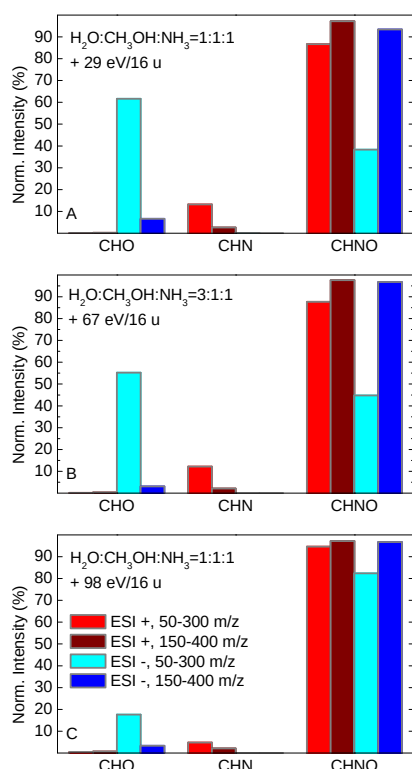
Fig. 5. Weighted abundance of CHO, CHN, and CHNO molecular groups in organic refractory residues. Panel A: 1:1:1 + 29 eV/16 u residue; panel B: 3:1:1 + 67 eV/16 u residue; panel C: 1:1:1 + 98 eV/16 u residue. Red and dark red columns refer to the analysis in positive ESI mode in the 50–300 and 150–400 m/z, respectively, while light blue and blue refer to the analysis in negative ESI mode in the 50–300 and 150–400 m/z range, respectively.
