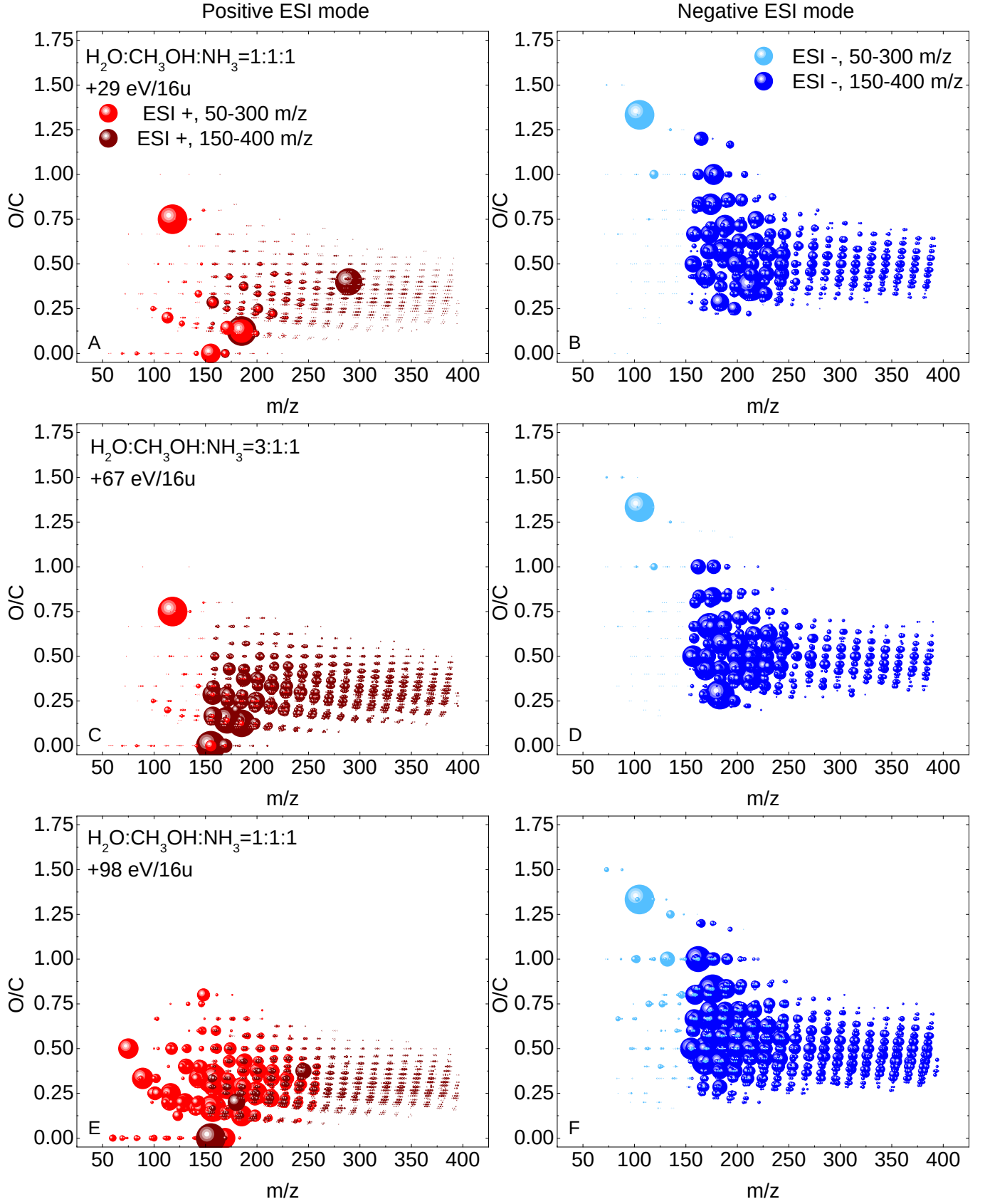
Fig. B.2. Ratios of O/C with respect to the m/z ratio in the range 50–300 and 150–400 m/z in positive ESI mode (left panels) and negative ESI mode (right panels). Panels A and B: 1:1:1 + 29 eV/16 u residue; panels C and D: 3:1:1 + 67 eV/16 u residue; panels E and F: residue of the 1:1:1 + 98 eV/16 u. The size of the dots is given by the normalized intensity.
