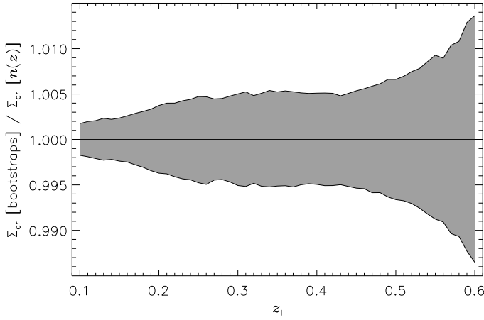
Fig. A.1. Relative errors in \Sigma_{cr} , estimated using 10^4 bootstraps of the spectroscopic catalog of Hildebrandt et al. (2017). The relative error on the ESD is negligible.
