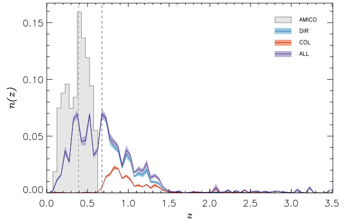
Fig. 4. Redshift distribution of AMICO clusters (gray), with a median redshift of z_l = 0.38 (dashed gray), and KiDS-450 background sources (purple), with a median redshift of z = 0.68 (dashed purple). In blue (DIR), we show the initial selection following Hildebrandt et al. (2017) and Dvornik et al. (2017) . In red, we show the estimated redshift distribution of the gri color selection (COL), corresponding to the bottom panel of Fig. 5.
