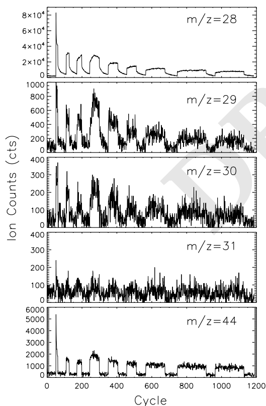
Fig. 2. Ion current vs cycle detected by the mass spectrometer during the nine irradiation steps for the parent molecules m/z = 28 (CO) and 31 (CH 3 OH), and for the main products of the top layer HCO, H 2 CO, CO 2 ( m/z = 29, 30 , and 44). The increase of the desorption at the fourth irradiation step marks the contribution of the bottom layer.
