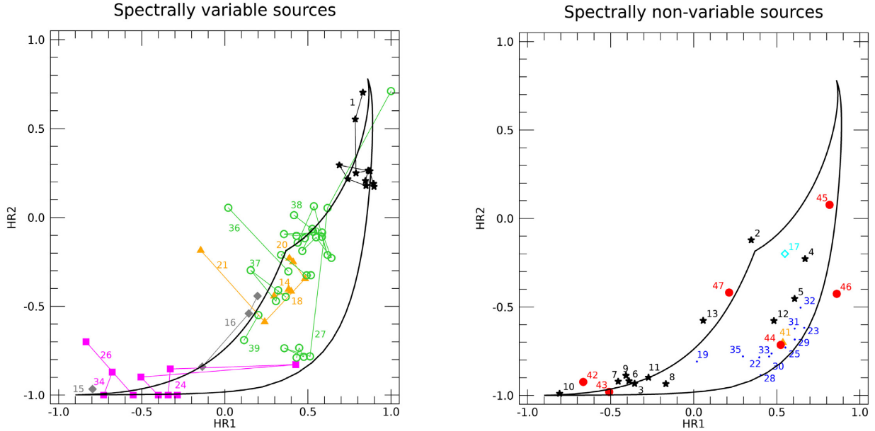
Figure 3. The HR_1 – HR_2 plane of the 47 soft sources divided into spectrally variable (left-hand panel) and non-variable (right-hand panel). They are numbered according to Table 3, and coloured according to their class: INSs (black stars), LMXBs and HMXBs (orange triangles), SNRs (blue small dots), SSSs (magenta squares), TDEs (grey diamonds), AGNs (cyan empty diamonds), and ULXs (green empty dots). The sources of unknown classification are represented by red dots.
