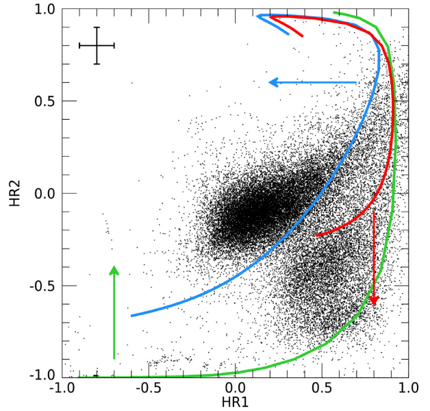
Figure 1. \text{HR}_1 – \text{HR}_2 plot of the point-like 4XMM-DR10 sources with errors on the hardness ratios smaller than 0.1 ((the error bars in the top left-hand corner illustrating this uncertainty)). The sources cluster into two main groups: The AGNs, having a non-thermal spectrum, are placed to the left of the blue line (POWERLAW, \Gamma \lesssim 4 ); the stars, having a thermal spectrum, are placed in the region below the red line indicated by the arrow (APEC, kT \lesssim 1.05 \text{ keV} , 0.5 solar abundance). The green line represents a blackbody (BBODYRAD) of temperature kT = 0.05 \text{ keV} ; typical INSs and super-soft sources (SSSs), with temperatures in the range of 0.05–0.25 keV, can be found in the region above this line indicated by the green arrow. The lines are obtained by varying N_{\text{H}} from 0 to 10^{23} \text{ cm}^{-2} using the TBABS model.
