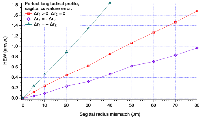
Figure 5: degradation of the HEW due to radius error in the sagittal (azimuthal) plane, for a perfect longitudinal profile. Besides the sole parabola error effect (red line, as in Figure 4), opposite errors in the parabola and the hyperbola (purple) compensate the aberration, while curvature errors with the same sign make it approx. double.
