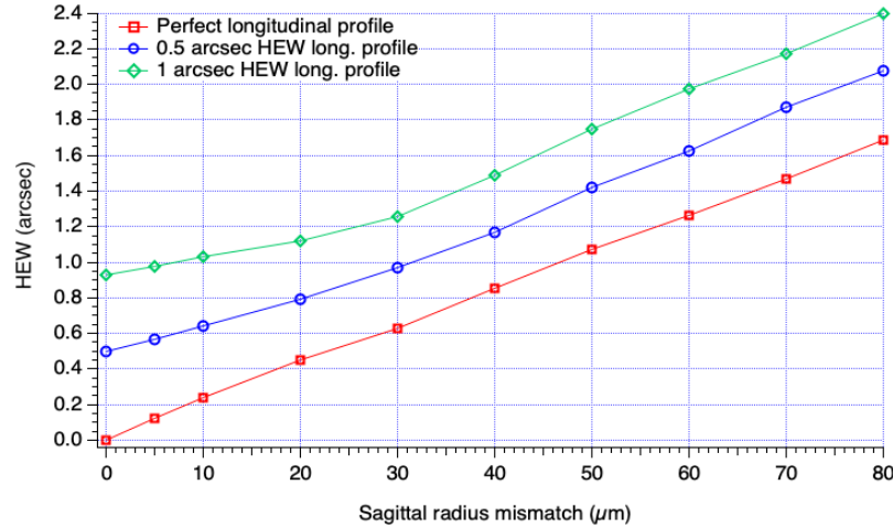
Figure 4: degradation of the HEW due to radius error in the sagittal (azimuthal) plane, for different values of the longitudinal error HEW. Only the parabolic segment error was simulated, while the hyperbola is assumed as perfect. The behavior of an error in the sole hyperbolic segment would be totally analogous.
