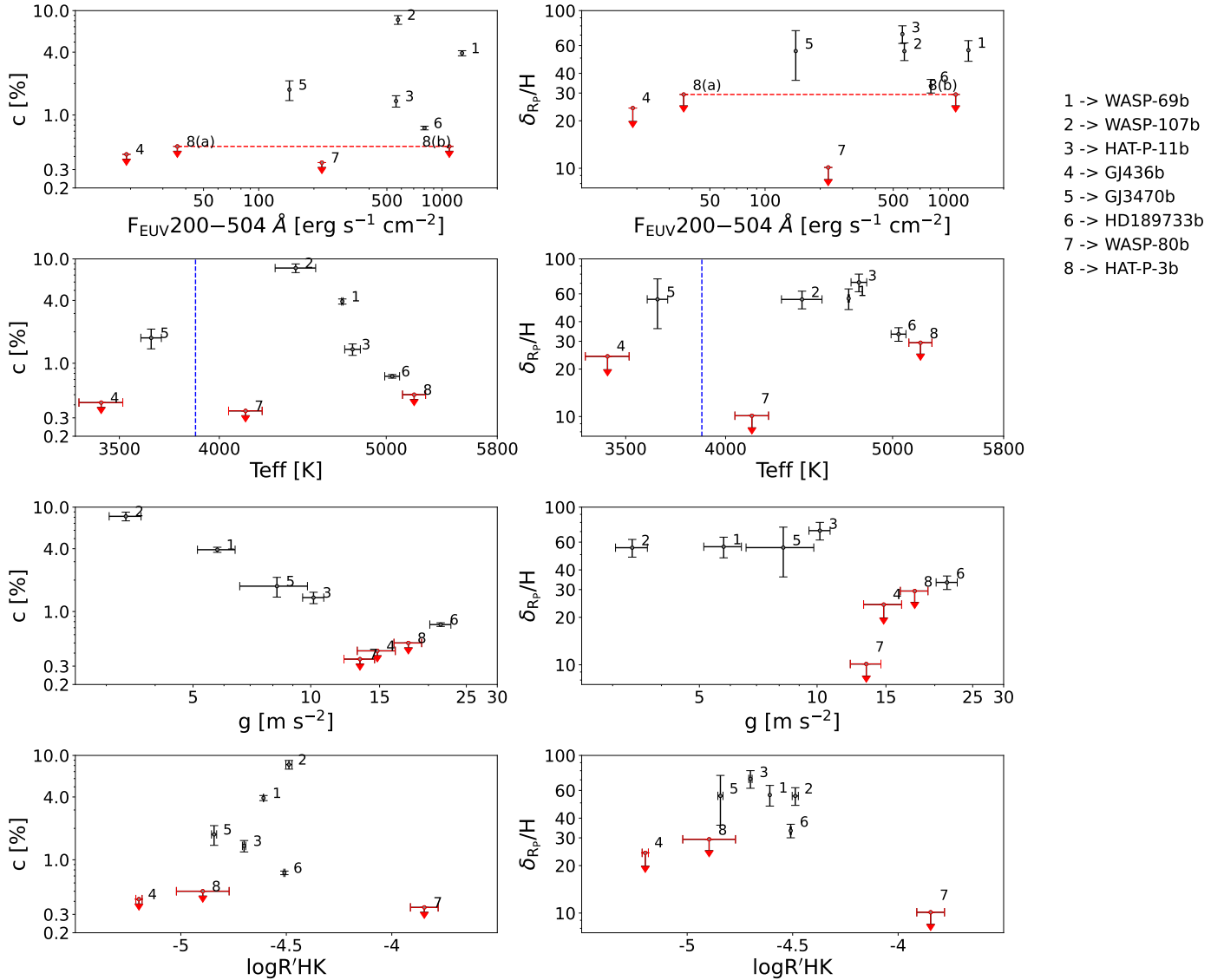
Fig. 8. Correlation plots. Targets are from this work, Guilluy et al. (2020, 2023) , and Fossati et al. (2022) . Contrast c (left panels) and \delta_{R_p}/H_{eq} (right panels) as a function of the EUV flux in the 200–504 Å range, effective temperature and planetary gravity, and \log R'_{HK} . Red markers indicate targets with only an upper limit on the He I detection (reported at 1\sigma ). The vertical dashed blue lines in the effective temperature diagrams indicate the transition from M-type to K-type stars. The dashed horizontal line connects the two possible locations for HAT-P-3b (for the two different coronal temperatures).
