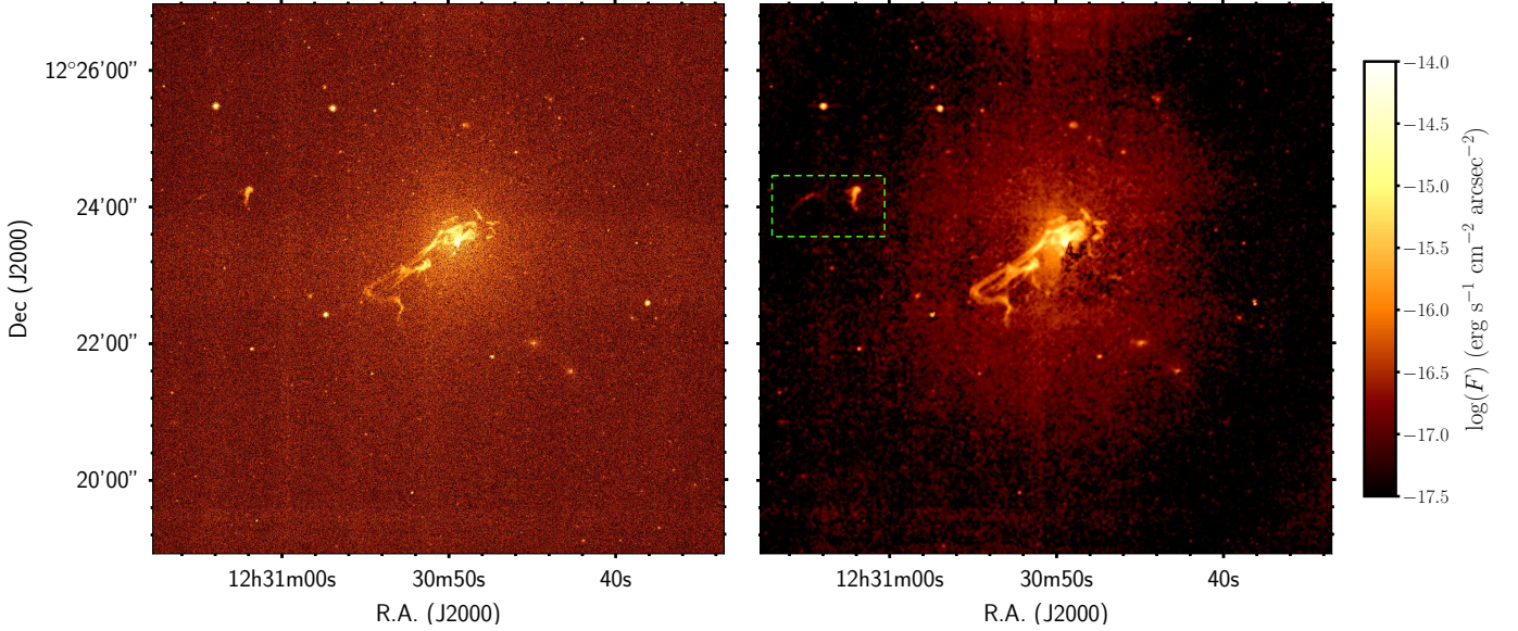
Fig. 1. Left panel: continuum-subtracted H\alpha + [NII] image of M87 at full resolution. Right panel: continuum-subtracted H\alpha + [NII] image of M87 after a 15 \times 15 boxcar smoothing, corresponding to \approx 2.8 arcsec resolution. At the distance of M87 (16.5 Mpc), 1 arcsec = 80 pc. The green dashed box indicates the zoomed-in region in Fig. 4. Smoothing reduces the noise in the outer parts, where the surface brightness sensitivity reaches \Sigma(H\alpha + [NII]) \approx 5 \times 10^{-18} \text{ erg s}^{-1} \text{ cm}^{-2} \text{ arcsec}^{-2} .
