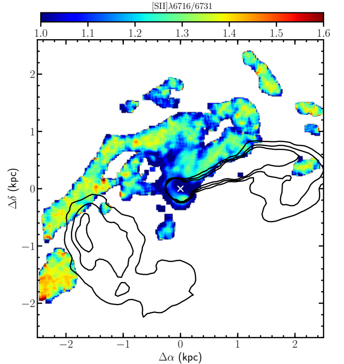
Fig. 8. Distribution of the [SII]\lambda 6716 \text{ \AA} / [SII]\lambda 6731 \text{ \AA} ratio for emission lines with a S/N > 5 .
