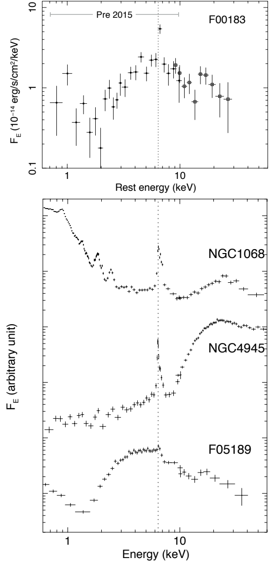
Fig. 6. Broad-band X-ray spectra of IRAS F00183–7111 and three obscured AGN with different degrees of absorption for a comparison: NGC 1068, a (cold) reflection-dominated spectrum without a transmitted component of the obscured nuclear source ( N_H \geq 10^{25} \text{ cm}^{-2} ); NGC 4945, a reflection-dominated spectrum below 10 keV with a transmitted component of the central source emerging above 10 keV ( N_H \sim 3.5 \times 10^{24} \text{ cm}^{-2} ); IRAS F05189–2524, moderately absorbed nuclear source ( N_H \sim (6\text{--}9) \times 10^{22} \text{ cm}^{-2} ). The 0.6–8 keV data for IRAS F00183–7111 are obtained by combining the XMM-Newton , Chandra and Suzaku data. For the other three, XMM-Newton data are used for the 0.6–10 keV band. Their spectra at higher energies are all obtained from NuSTAR . All the comparison spectra show Fe K emission peaking at 6.4 keV as indicated by the dotted line whereas that in IRAS F00183–7111 peaks at 6.7 keV (see Sect. 3.2.1). NGC 1068 and NGC 4945 exhibit excess features in the NuSTAR band due to a cold reflection hump and an absorbed component, respectively.
