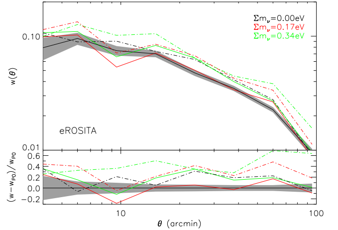
Figure 10. Correlation function as a function of the angular separation for the haloes detectable by the eROSITA cluster survey (see text for details). The grey-shaded area shows the Poissonian error ( 1\sigma ) for the P0 simulation only computed over the 50 light cones ( 5000 \text{ deg}^2 ). In the lower subpanel we show the fractional difference computed with respect to the P0 simulation.
