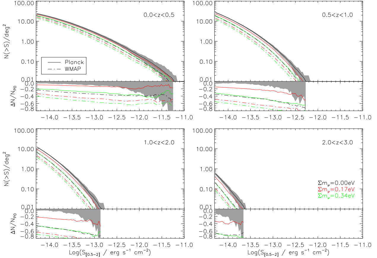
Figure 8. Same as Fig. 3, but for the number of galaxy clusters as a function of limit flux in the 0.5–2 keV band.
