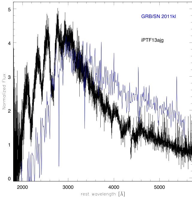
Figure 7. The maximum-light spectrum of GRB/SN 2011kl (blue line) compared to that of iPTF13ajg (black line).
