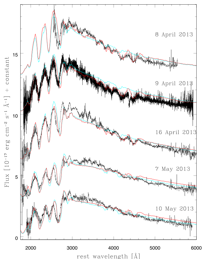
Figure 3. The pre- and near-maximum spectra of iPTF13ajg, compared to synthetic spectra. One of the model series (cyan) does not include an increase in the occupation numbers of \text{O II} and \text{He I} to account for non-thermal effects, while the other (red) does.
