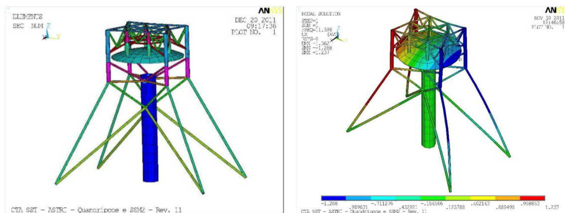
Figure 3.1 (left) FEM of the mast structure. (right) Evaluation of the Eigen-modes.
