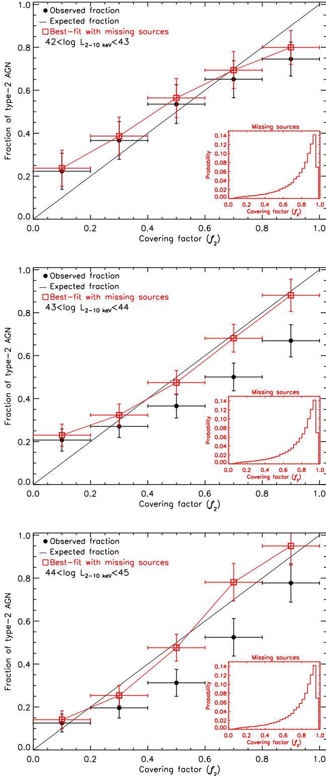
Figure 1. Type-2 AGN fraction vs. torus covering factor f_2 for objects with 10^{42} < L_X < 10^{43} (top), 10^{43} < L_X < 10^{44} (middle), and 10^{44} < L_X < 10^{45} erg s ^{-1} (bottom). Filled circles are the observed type-2 AGN fractions in BUXS. Open squares are the best-fit models to the 1:1 relations (black solid lines) obtained by allowing a population of non-detected type-2 sources. The insets show the assumed f_2 distribution of these missed sources.
