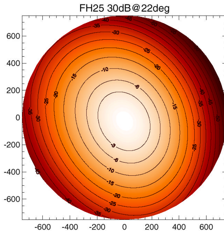
Fig. 3-14: Feed Horn # 25: Field Distribution on the main reflector
