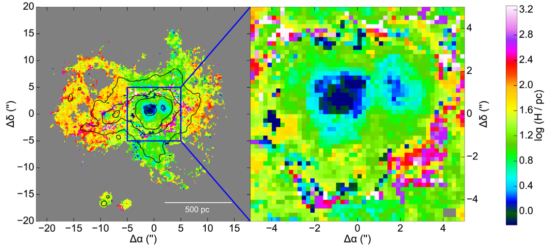
Figure 4. Left panel: ‘effective’ scale height defined as H = N_H/n . As in Fig. 1, black lines show the contours of the H \alpha emission line (80, 10, 4, and 1 in units of 10^{-16} erg s ^{-1} cm ^{-2} ). Right-hand panel: zoom on the blue box.
