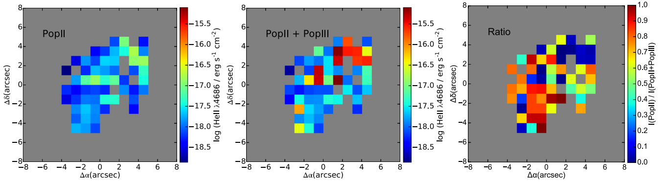
Figure 18. Predicted He II \lambda 4686 line emission by GAME for the spaxels of IZw18 using, respectively, the library containing only PopII stars (left-hand panel), and the full library containing also the contribution from PopIII (central panel). Right-hand panel: ratio between the predicted intensities in the left and central panels showing a negligible contribution from PopII stars in the NW region.
