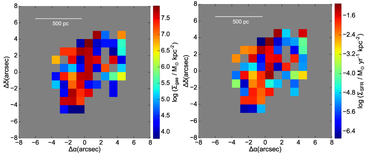
Figure 16. Gas mass surface density ( \Sigma_{\text{gas}} , left-hand panel) and star formation surface density ( \Sigma_{\text{SFR}} , right-hand panel) for the galaxy IZw18.
