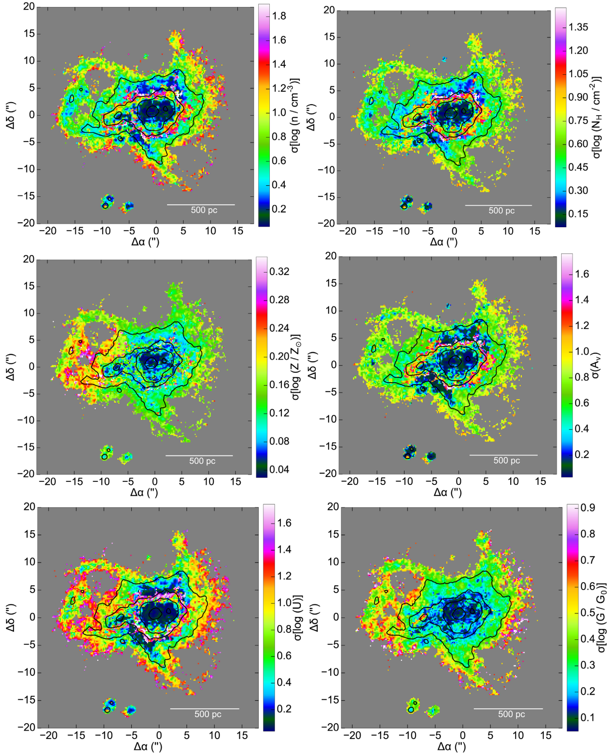
Figure B1. Relative uncertainties on the He 2-10 ISM physical properties reported in Fig. 2: density ( n ), column density ( N_{\text{H}} ), metallicity ( Z ), visual extinction ( A_{\text{V}} ), ionization parameter ( U ), and the FUV flux in the Habing band ( G/G_0 ). As in Fig. 1, black lines show the contours of the \text{H}\alpha emission (80, 10, 4, and 1 in units of 10^{-16} \text{ erg s}^{-1} \text{ cm}^{-2} ). In the upper left corner, we report the average relative uncertainty on the inferred values.
