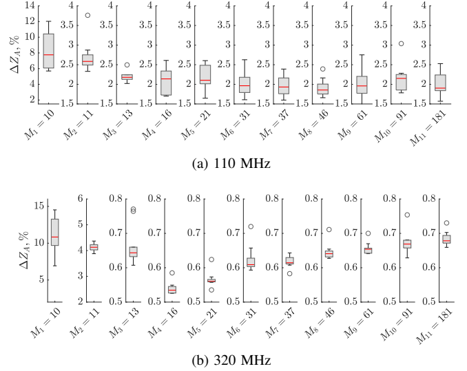
Fig. 7. Relative error of \mathbf{Z}_A for M sample points in EEP data: (a) 110 MHz and (b) 320 MHz. Box and whiskers plots show the statistical indicators of 10 Monte-Carlo runs. EEPs are within the field of view, \theta \in [-45^\circ, 45^\circ] .
