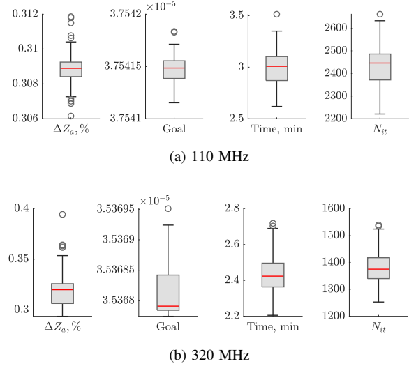
Fig. 4. Box and whiskers plots show statistical indicators of 100 Monte-Carlo runs for \mathbf{Z}_A (10), goal function (8), overall extraction time in minutes and number of iterations. Red lines show mean values. The EEPs contained M = 361 samples within \theta \in [-90^\circ, 90^\circ] .
