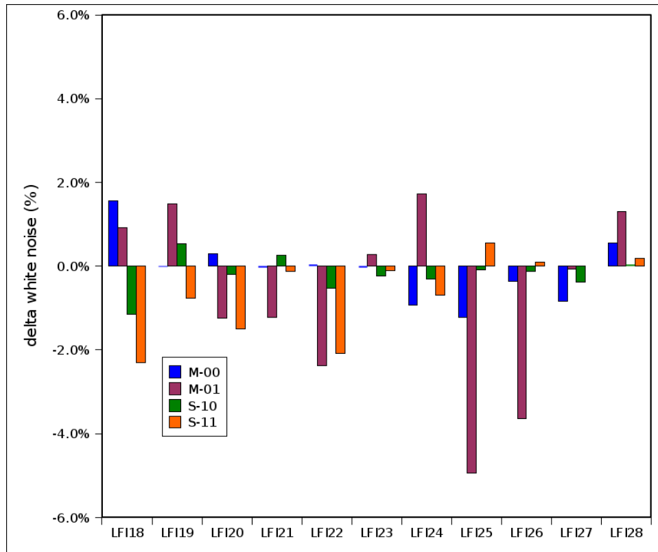
Figure 9 - Percent variation in uncalibrated white noise between the two phase switch configurations. The variation in LFI23 can be considered as a reference for the repeatability of this comparison, as LFI23 did not change configuration in the two acquisitions
