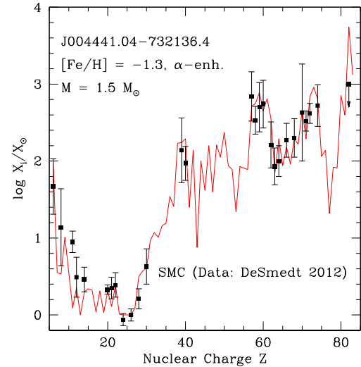
Figure 23. Comparison of our model results with the observations for the post-AGB star J004441.04–732136.4. See text for details.
