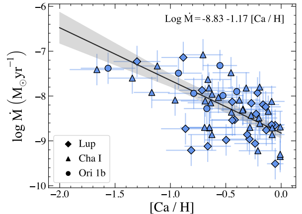
Figure 4. [\text{Ca}/\text{H}] vs \text{Log}(\dot{M}) . The black line represents the best fit from the MCMC linear regression; our 1\sigma confidence intervals are shown in gray.
