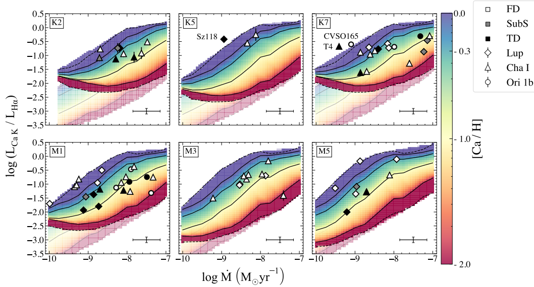
Figure 1. Comparison of \log(L_{\text{CaIIK}}/L_{\text{H}\alpha}) vs. accretion rate between magnetospheric accretion models (background) and observations (dots). Models are colored by [\text{Ca}/\text{H}] , with purple representing solar abundance (1) and depletion increasing toward red. The gray-out region represents the magnetospheric models without the contribution of the WTTS. Solid lines represent the median value for a given model abundance (1, 0.5, 0.1, 0.01) and dashed lines represent the 16% and 84% percentiles for the lowest and highest abundance values of the models, respectively. Typical uncertainties for observations are shown in the lower right corner.
