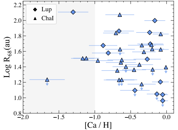
Figure 7. [\text{Ca}/\text{H}] vs R_{68} . No relationship between R_{68} and [\text{Ca}/\text{H}] is found.
