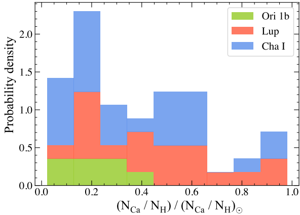
Figure 2. Probability density of the abundance by number, colored by star-forming region.
