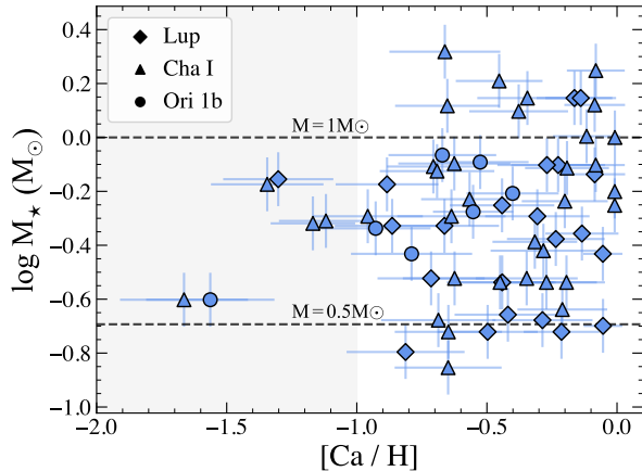
Figure 3. [\text{Ca}/\text{H}] vs. M_* . The grey region highlights the [\text{Ca}/\text{H}] \leq -1 region, the minimum abundance we are able to detect for M_* > 1 . No relationship between the stellar mass and Ca abundance is found.
