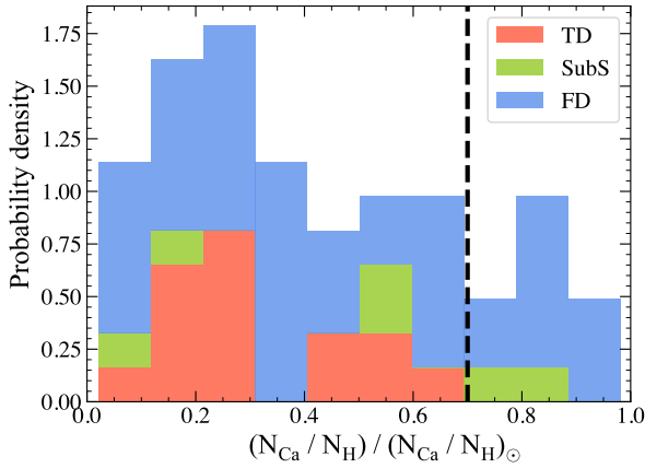
Figure 5. Probability density of abundance by number, colored according to the presence of gaps (red, TD), substructures (green, SubS), or absence of both (blue, FD) in each system. The black dashed lines represents (N_{\text{Ca}}/N_{\text{H}}) / (N_{\text{Ca}}/N_{\text{H}})_{\odot} = 0.7 .
