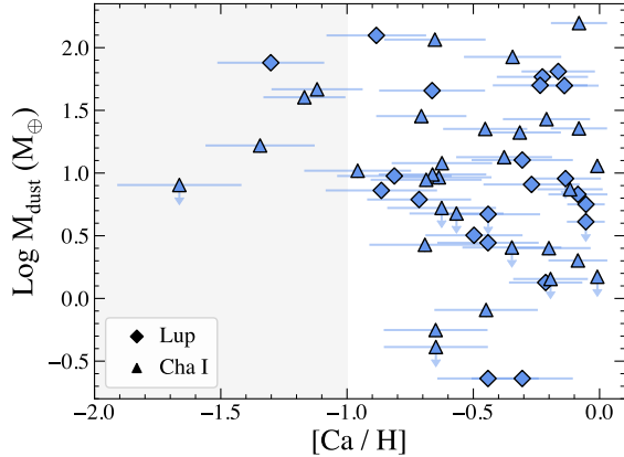
Figure 6. M_{\text{dust}} vs. [\text{Ca}/\text{H}] . Upper limits are indicated as arrows. No relationship between M_{\text{dust}} and [\text{Ca}/\text{H}] is found.
