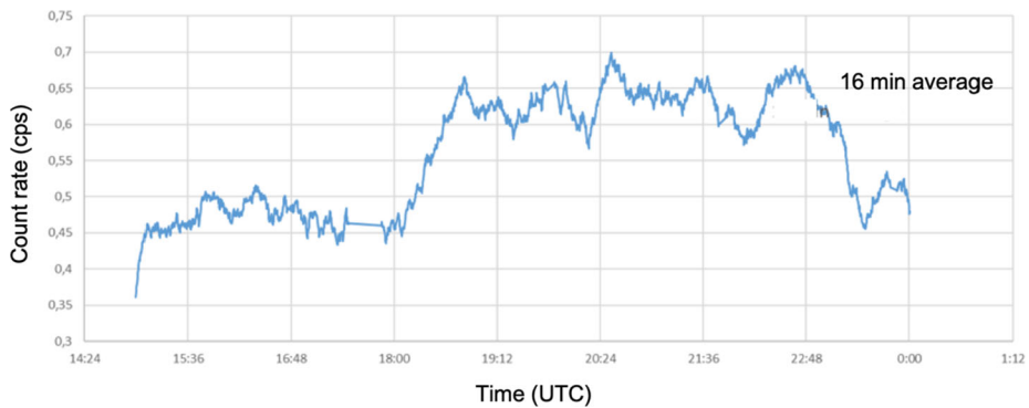
Fig. 21 SIXS-X detector 1, 16 min sliding average raw count rate including channels between 1–2 keV on June 4th 2019. Spacecraft slew maneuver was initiated at 17:57 and completed at 18:47 (UTC). Slew reversion began at 22:57 and ended at 23:47. Increased count rate during the maneuver beginning from about 18:00 is due to the emergence of the Sun in the detector's FoV. The background count rate of 0.45–0.5 cps is primarily due to the low energy tail from the in-flight calibration source in the spectral window
