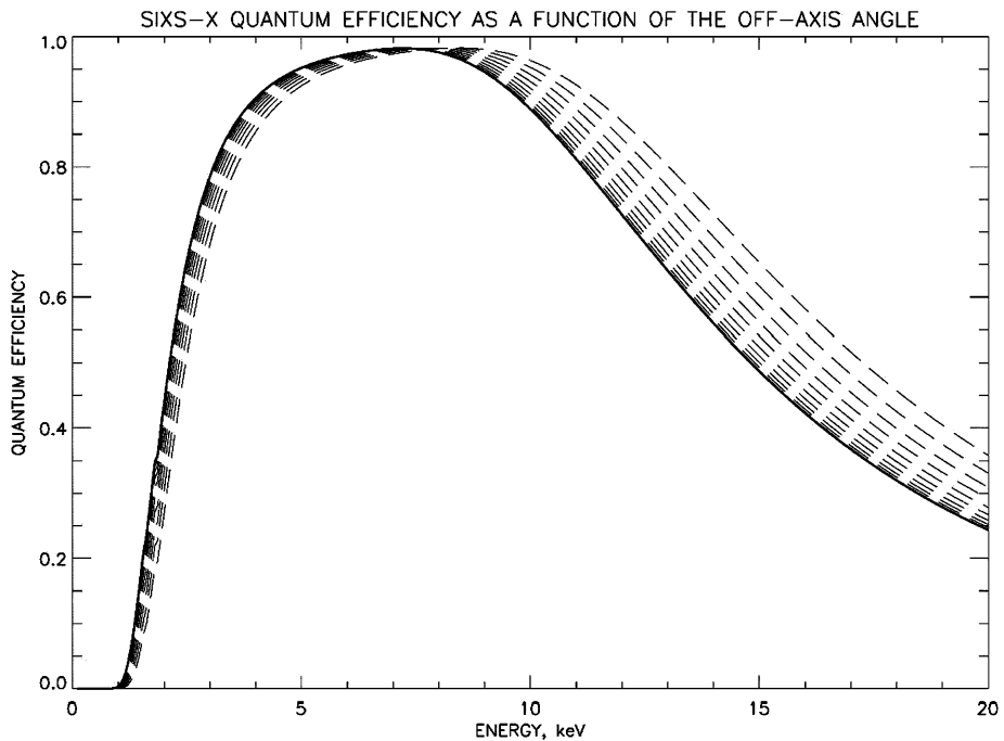
Fig. 12 Quantum efficiencies of the SIXS-X detectors as a function of photon energy plotted with off-axis angles between 0^{\circ} – 55^{\circ} with 5^{\circ} steps
