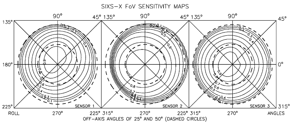
Fig. 13 Relative FoV sensitivity maps of the SIXS-X detectors normalized to maximum (on-axis) FoV sensitivity
