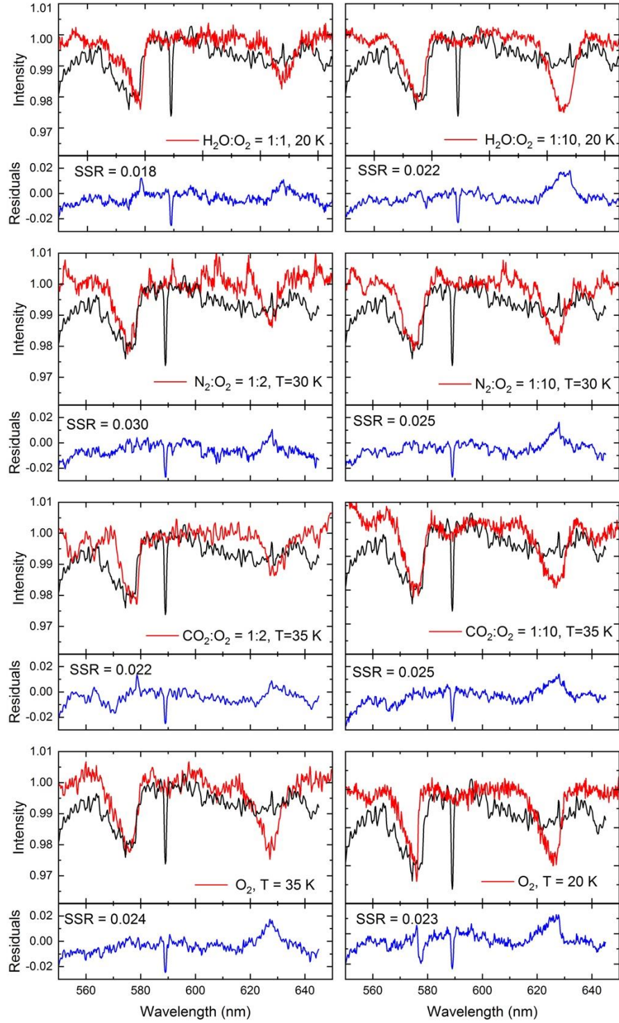
Fig. A1. Ground-based spectrum of Ganymede acquired in reflectance at TNG (black curve) compared to selected laboratory transmittance spectra of solid O 2 , pure and mixed with H 2 O, CO 2 , and N 2 , with different mixing ratios and ice temperatures (in red). Blue lines are the spectral residue that is the difference between black and red lines. SSR stands for sum of squared residuals.
