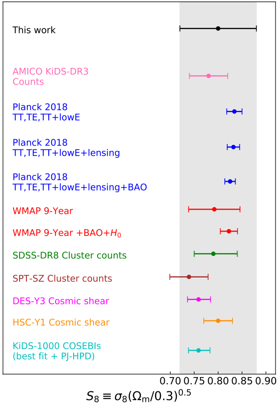
Fig. 4. Comparison of the constraints on S_8 \equiv \sigma_8(\Omega_m/0.3)^{0.5} obtained, from top to bottom, from the cluster clustering analysis in the AMICO KiDS-DR3 catalogue (black dot), from the joint analysis of cluster counts and weak lensing in KiDS-DR3 performed by Lesci et al. (2022, pink dot), from the results obtained by Planck Collaboration VI (2020, blue dots), Hinshaw et al. (2013, red dots), Costanzi et al. (2019, green dot), Bocquet et al. (2019, brown dot), Amon et al. (2022) and Secco et al. (2022, magenta dot), Hikage et al. (2019, orange dot), and Asgari et al. (2021, cyan dot). The median and the 16th and 84th percentiles are shown.
