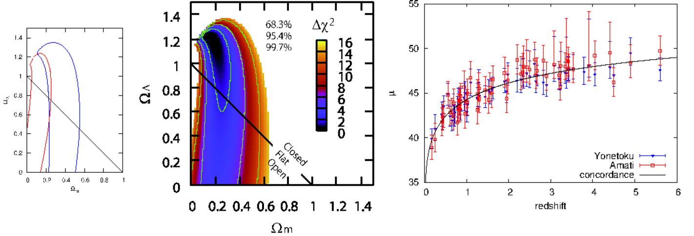
Figure 6. Left panel: constraints on \Omega_M , \Omega_\Lambda from the Amati (red) and Yonetoku (blue) relations (Tsutsui et al. 2009a). The contours correspond to 68.3% confidence regions; black solid line represents the flat universe. The results are consistent on the 2\sigma level. Middle panel: Constraints on \Omega_M , \Omega_\Lambda the from E_{\text{peak}} - T_L - L_{\text{peak}} relation (Tsutsui et al. 2009a). Right panel: extended HD from the Amati (red) and Yonetoku (blue) relations (Tsutsui et al. 2009a). A systematic difference is apparent in high- z GRBs, although it does not seem to be present in low- z ones.
