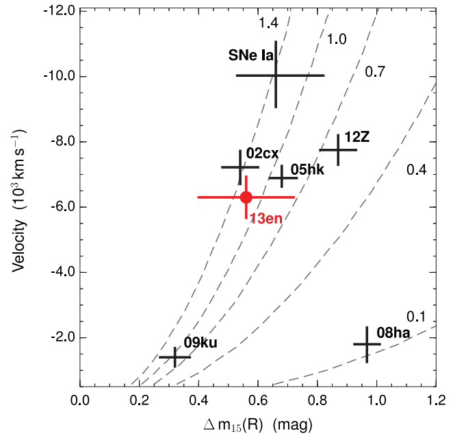
Figure 8. Comparison of \Delta m_{15}(R) and the photospheric velocity at around the maximum light ( t \approx +3 d) for various objects in the SN 2002cx-like class. The dashed lines represents the relationship between ejecta velocity and \Delta m_{15} for (from bottom right to top left) 0.1, 0.4, 0.7, 1.0 and 1.4 M_{\odot} of ejecta mass. SN 2013en is marked with a red filled circle.
