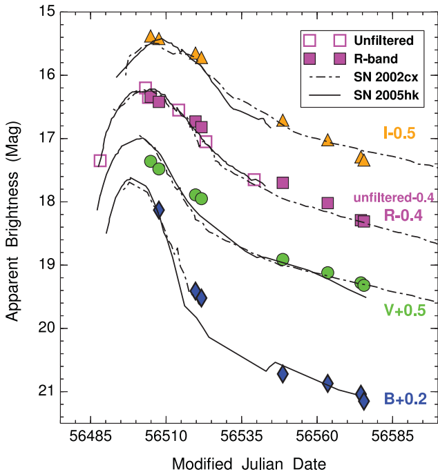
Figure 2. BVR (filled markers) and unfiltered (open squares) light curves (LCs) of SN 2013en. The LCs have been shifted by the amount indicated in the legend. For a comparison, the LCs of SNe 2002cx ( BVR band, dash-dotted lines) and 2005hk ( BVR band, solid lines) are also shown. The LCs of SNe 2002cx and 2005hk have been shifted to match the light curve of SN 2013en at peak. Here, the uncertainties for data points are smaller than the plotted symbols.
