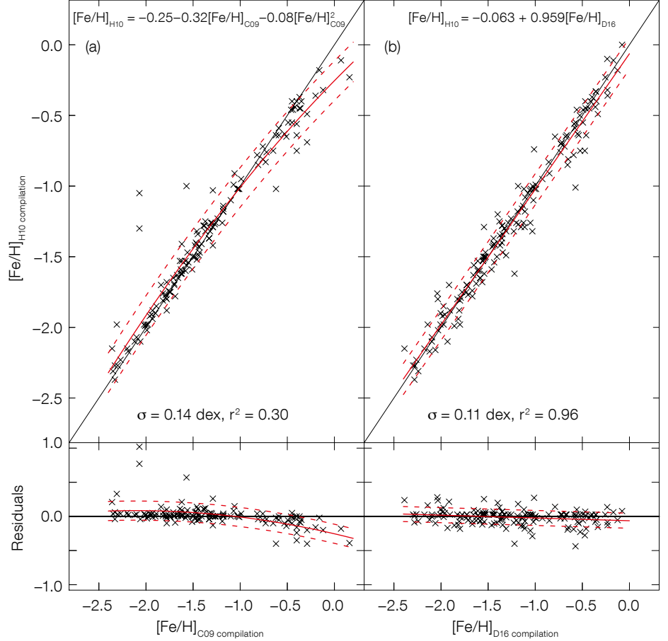
Figure 2. (a) Comparison of metallicities of 132 clusters common to the metallicity scales of Carretta et al. (2009) and Harris (1996), C09 and H10 respectively. The best fit and 1\sigma limits are shown by red continuous and dotted lines, respectively. (b) The same as (a) but for 151 clusters common to our abundance scale (Dias et al., 2016a) and that of Harris (1996). Details of the fits are given in each panel.
