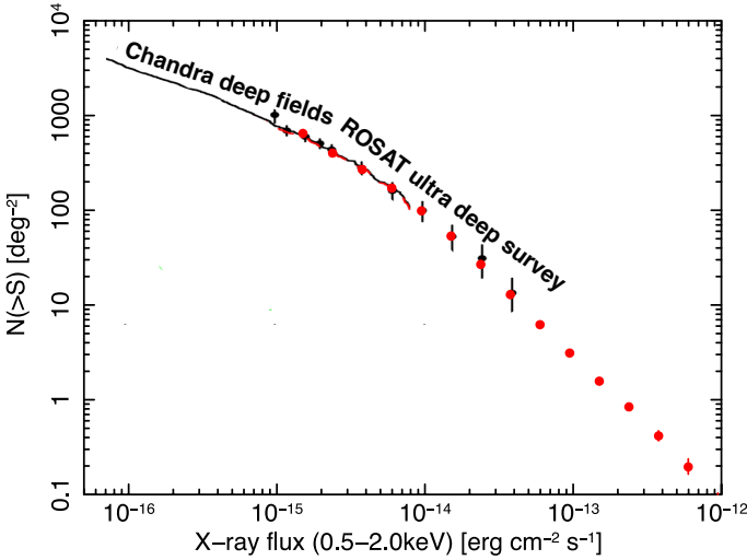
Fig. 6. A comparison of the 0.5-2.0 keV X-ray LogN-LogS of our Survey (red points) with that measured by Chandra (solid line) and ROSAT (black filled circles). Adapted from Brandt & Hasinger (2005).
