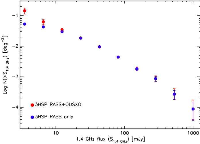
Fig. 8. The radio LogN-LogS of HBL blazars estimated using the sub-sample of 3HSP blazars included in the RASS (blue filled circles) and that of the combined OUSXG and RASS samples (red filled circles). A significant level of incompleteness is clearly present in the 3HSP sample below \sim 20 mJy
