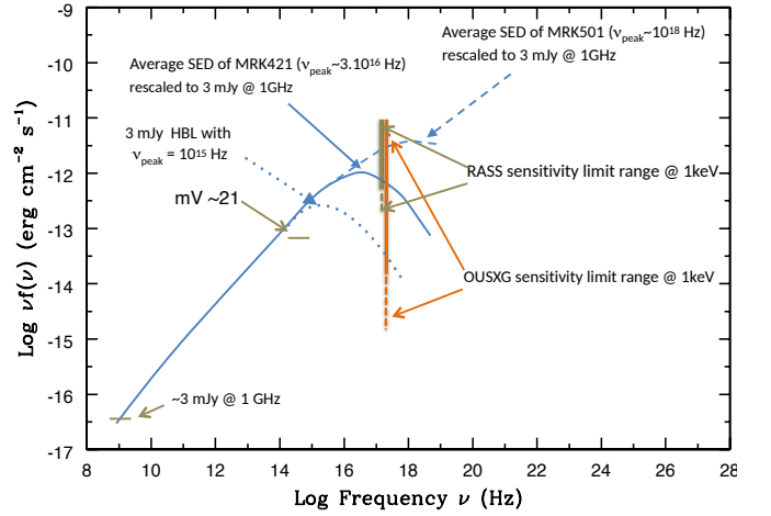
Fig. 7. Simple scheme comparing the sensitivity ranges of the RASS and the OUSXG surveys at \sim 1 \text{ keV} to the SED of different types of HBL blazars with radio flux density of 3mJy, close to the sensitivity limit of existing radio surveys. Blazars of this radio flux-density and \nu_{\text{peak}} \lesssim 10^{16} \text{ Hz} can only be detected in the OUSXG survey and are therefore missing in catalogues that require detection in the RASS.
