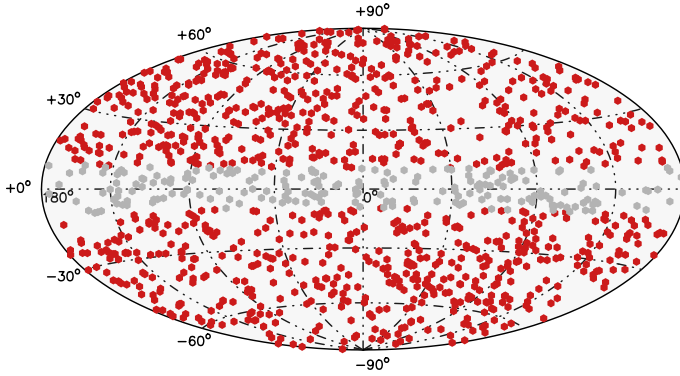
Fig. 1. Hammer-Aitoff plot in Galactic coordinates of all the Swift-XRT fields centred on GRBs and observed in PC readout mode. The 1,046 fields at Galactic latitude larger than 10 degrees used for the extragalactic survey are shown in red.
