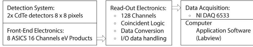
Fig. 3. Chain composing the prototype test system and the respective subsystems.
