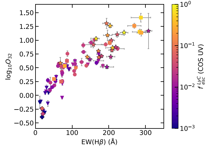
Figure 22. \text{O}_{32} vs. H \beta EW. Symbols are the same as in Figure 21. A strong correlation is evident, owing to the coupling of ionization parameter with starburst age.
