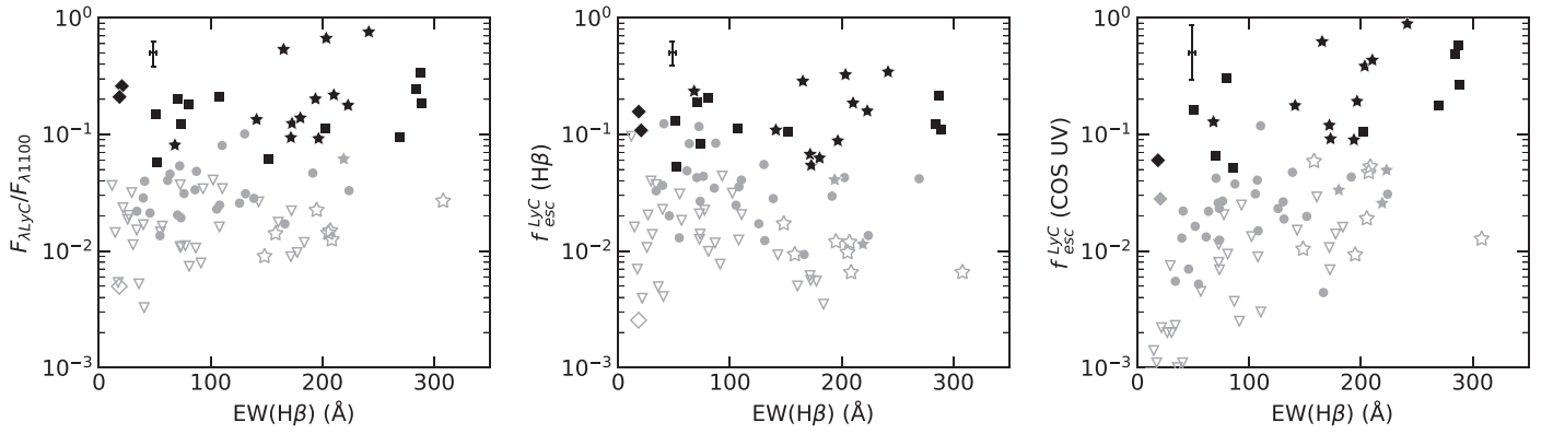
Figure 9. Same as Figure 1, but for the rest-frame H \beta EW.
