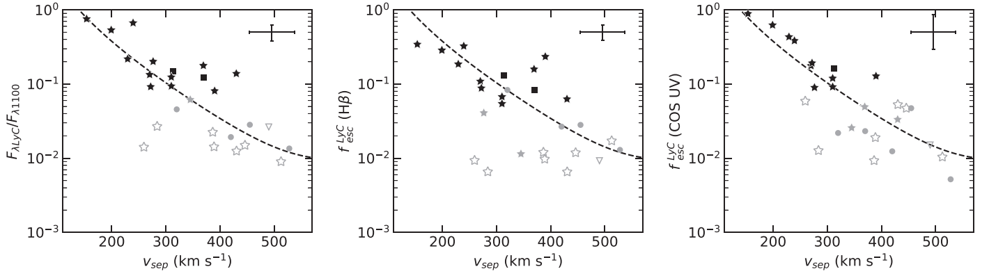
Figure 4. Same as Figure 1, but for Ly \alpha peak velocity separation v_{\text{sep}} . Results include only seven galaxies from the LzLCS plus the Izotov et al. (2016a, 2016b, 2018a, 2018b, 2021) samples. The dashed line is the description by Izotov et al. (2018b).
