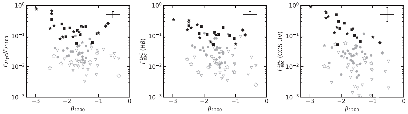
Figure 13. Same as Figure 1, but for the UV spectral index \beta_{1200} .
