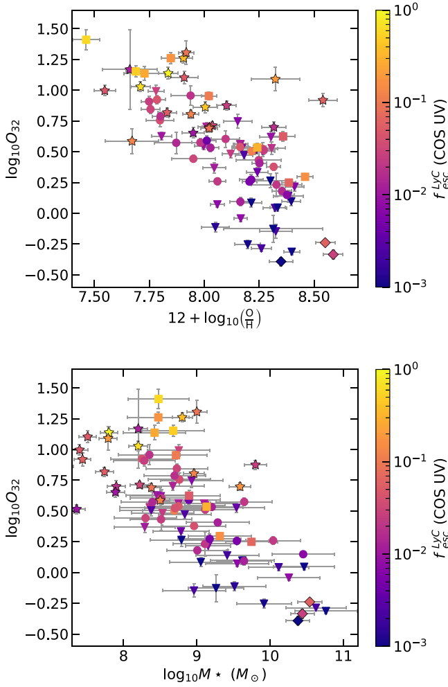
Figure 23. O_{32} compared to metallicity indicator 12 + \log_{10}(O/H) and SFH indicator M_* . Symbols are the same as in Figure 21.
