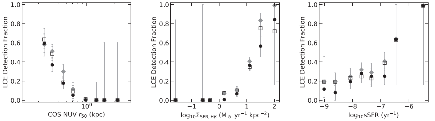
Figure 18. Same as Figure 2, but for r_{50} , \Sigma_{\text{SFR}} , and s\text{SFR} .
