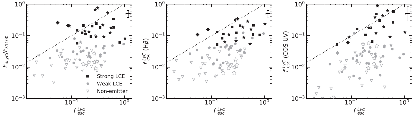
Figure 1. Comparison of F_{\text{LyC}}/F_{\lambda 1100} (left), f_{\text{esc}}^{\text{LyC}} from H \beta (middle), and f_{\text{esc}}^{\text{LyC}} from fitting the COS UV spectrum (right) with f_{\text{esc}}^{\text{Ly}\alpha} for strong LCEs ( >5\sigma LyC detection and f_{\text{esc}}^{\text{LyC}} > 0.05 ; filled black), weak LCEs ( >2\sigma LyC detection but not strong; filled gray), and nonemitters ( <2\sigma LyC detection; open gray). For nonemitters, f_{\text{esc}}^{\text{LyC}} is shown for the 1\sigma upper limit on the LyC flux. LzLCS results are shown as squares (strong LCEs), circles (weak LCEs), and triangles (nondetections), while the Izotov et al. (2016a, 2016b, 2018a, 2018b, 2021) galaxies are shown as stars and the Wang et al. (2019) galaxies are shown as diamonds. Characteristic 1\sigma uncertainties are shown in the upper right corner. The dotted line indicates 1:1 equivalence.
