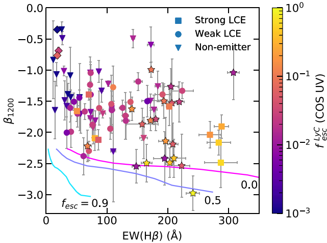
Figure 21. UV \beta_{1200} vs. H \beta EW for the LzLCS strong (squares) and weak (circles) LCEs and nonemitters (triangles) color-coded by f_{\text{esc}}^{\text{LyC}} derived from the UV spectrum. Solid lines are the Zackrisson et al. (2013) \sim 30\% solar-metallicity picket fence model predictions for f_{\text{esc}}^{\text{LyC}} = 0.0 (magenta), 0.5 (purple), and 0.9 (cyan). There appears to be no association of f_{\text{esc}}^{\text{LyC}} with a particular sequence in the UV \beta_{1200} –EW(H \beta ) plane. While symbols are color-coded by the UV-fit f_{\text{esc}}^{\text{LyC}} , the observed trends here and in subsequent figures are similar if one of the other f_{\text{esc}}^{\text{LyC}} metrics is used.
