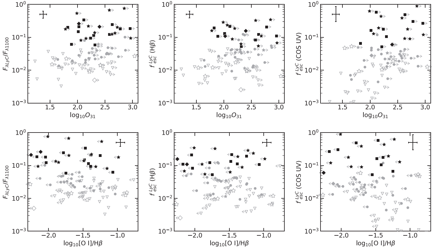
Figure 5. Same as Figure 1, but for O_{31} and [O\text{ I}]/H\beta .
