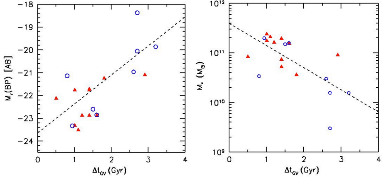
Figure 8. ( Left ) The absolute M_r magnitude reached at the Brightest Point of the rest-frame CMD diagram vs. the time spent in the GV, as defined in Section 4; the correlation (dashed line) index is 0.72, and the slope of the regression is 1.27. ( Right ) The total stellar mass at z=0 vs. the time spent in the GV; the correlation (dashed line) index is -0.67, and the slope of the regression is -0.45. Symbols are as in Fig. 7.
