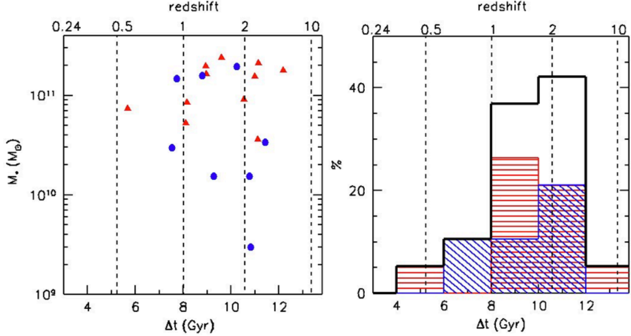
Figure 7. ( Left ) The total stellar mass at z=0 vs. age (either merger age or time of the onset of the SF due to galaxy flyby). The merger age ( \Delta t ) is the difference between the galaxy age at z=0 and that at the beginning of the merger (Section 4). (Red) triangles are the eleven galaxies studied in this paper, (blue) circles are the eight galaxies from Mazzei et al. (2014a). ( Right ) Histogram of the percentage of ETGs as a function of age (again, either merger age or time of the onset of the SF due to galaxy flyby). The horizontally shaded histogram is for galaxies in this paper, while the tilted one is for those in Mazzei et al. (2014a), both normalized to the total number of ETGs analyzed (19) (thick line).
