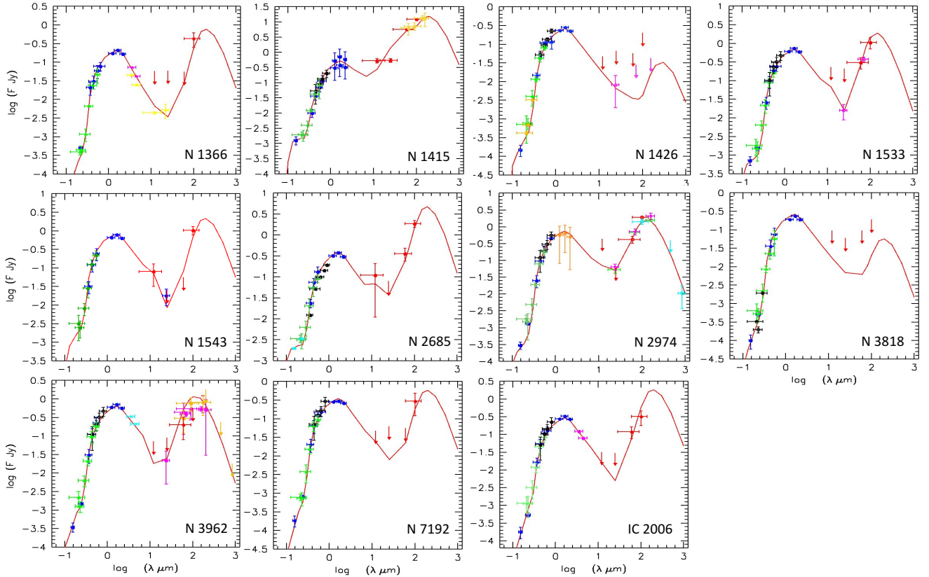
Figure 1. The SEDs of our targets (colored dots) compared with predictions from SPH-CPI simulations in Table 2 (red solid lines) at the galaxy ages in Table 3; green triangles are Swift -UVOT magnitudes from Paper II, blue filled circles are from NED, black dots from CGS catalogue (Ho et al. 2011; Li et al. 2011), and red points are IRAS fluxes from NED; other details are in Appendix. Data are corrected for our own galaxy extinction following prescription of NED and Paper II in the Swift -UVOT filters.
