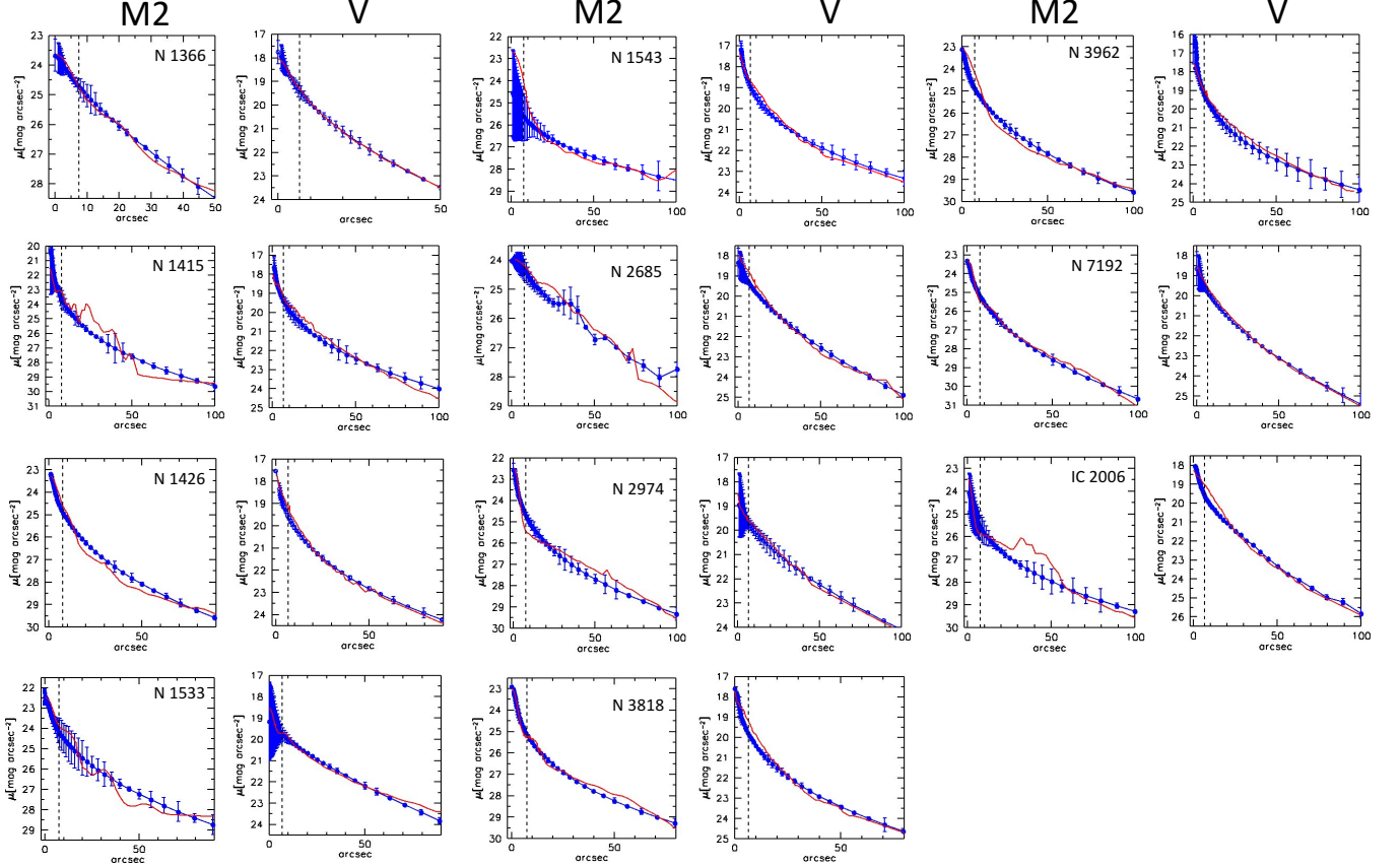
Figure 3. Luminosity profiles of our targets in the Swift -UVOT M2 and V bands; blue dots are Sérsic functions in Paper II, red solid lines are from the simulation snapshots in Fig.2.
