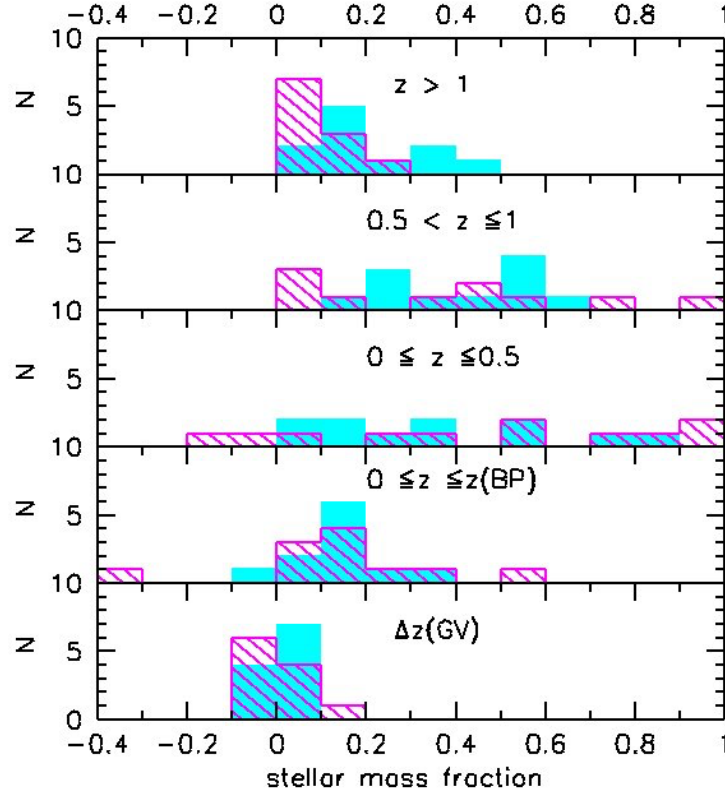
Figure 6. Number of galaxies vs the fraction of stellar mass assembled in different evolutionary steps within 50 kpc, (cyan filled, and R_{25} in Table 1, (magenta tilted). Accounting for cosmological parameters in Section 1, the look-back times to redshift 0.5 and 1 are about 5.2 and 8 Gyr respectively; BP and GV indicate the Brighter Point and the Green Valley of the CMD of each galaxy. NB: the negative fractions indicate mass loss in the interval considered.
