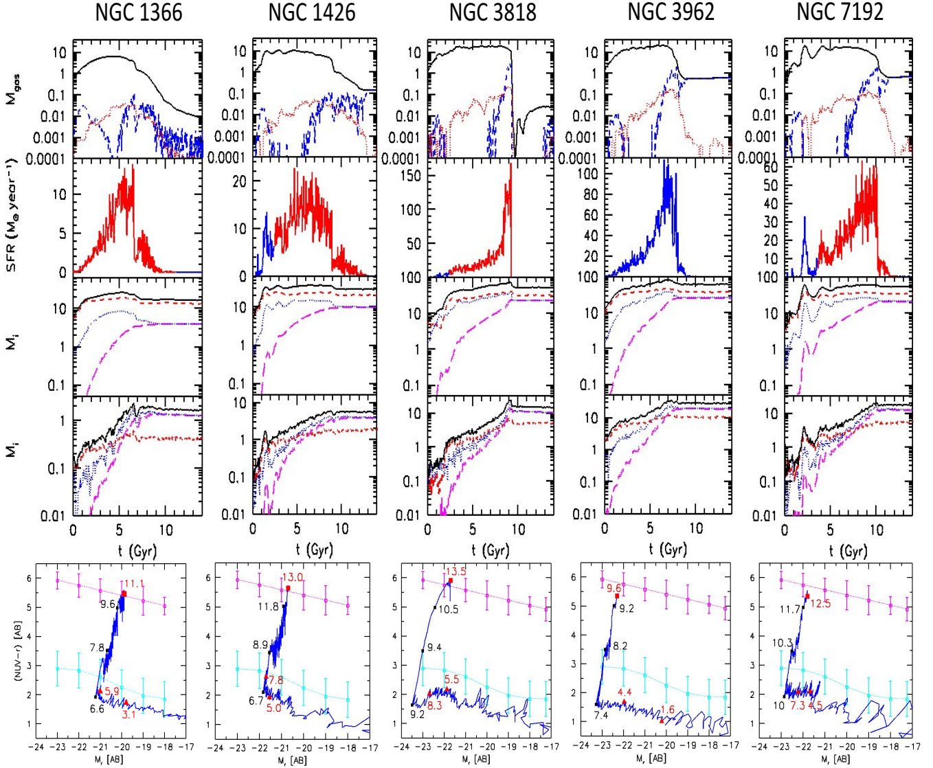
Figure 4. Evolutionary properties of ETGs without UV features. From top to bottom: the gas accretion history, the SFR (red line from the beginning of the merger as defined in Section 4), the mass assembly history (see also Table 4) within 50 kpc and R_{25} in Table 1, both centered on the B-band luminous center of the galaxy, and the CMD in the galaxy rest-frame; more details in Section 4. M_{\text{gas}} and the different mass components, M_i , are in units of 10^{10} M_{\odot} .
