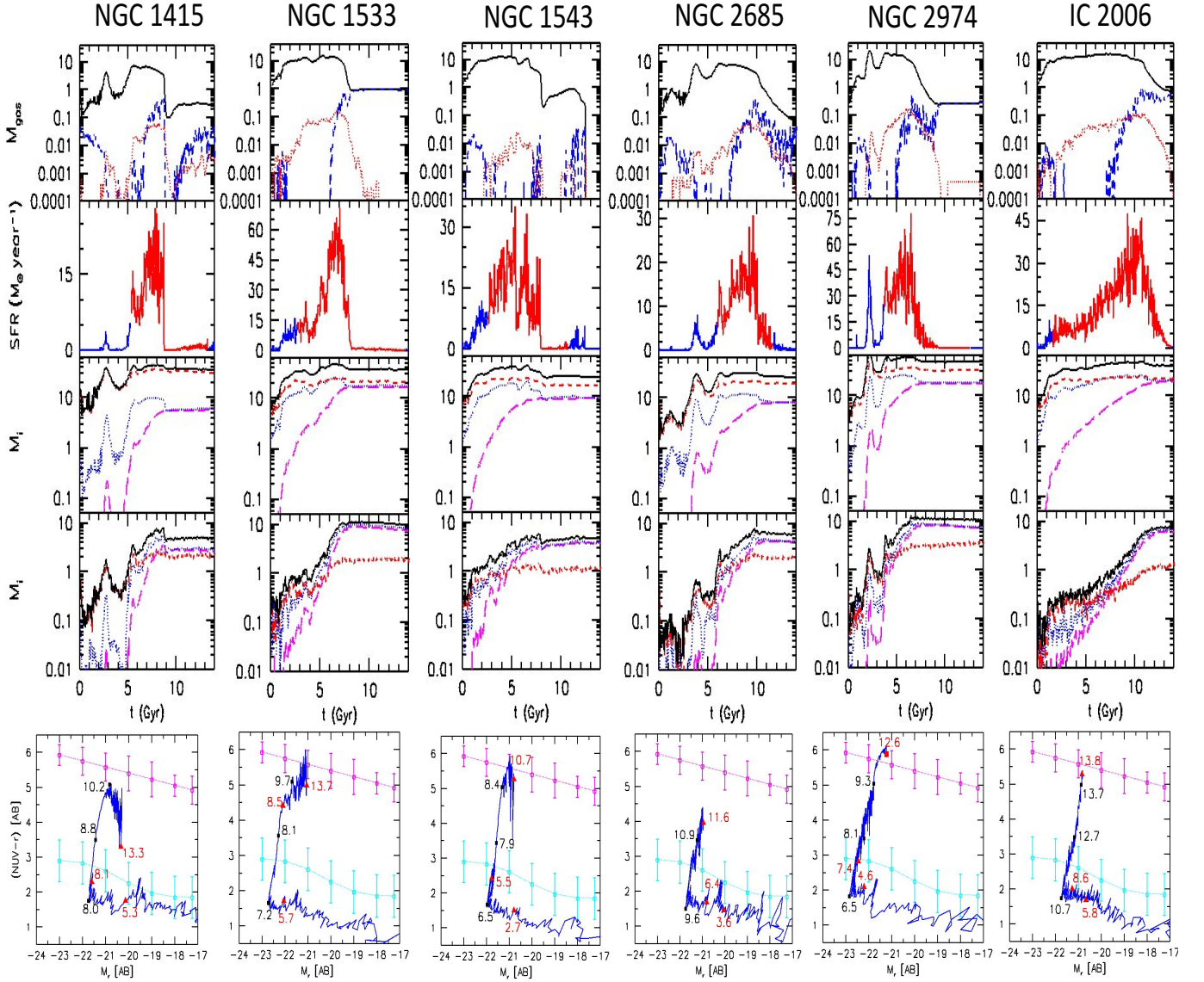
Figure 5. As in Fig.4 for ETGs with UV features.
