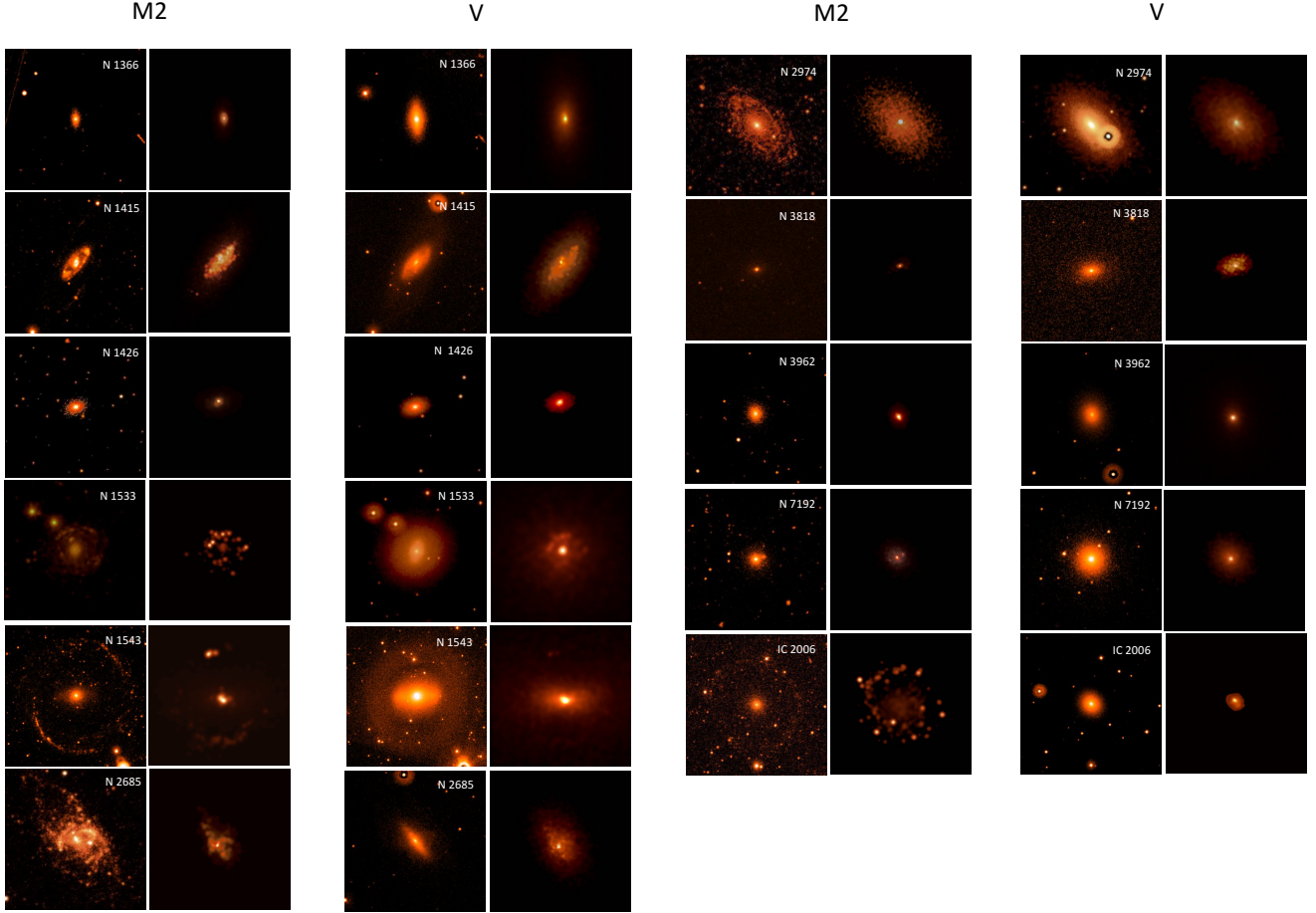
Figure 2. Observed vs. simulated image of the 11 galaxies. In each column: left : the Swift -UVOT M2 (cols 1, 5) or V (cols 3, 7) band image; right : the simulated image (cols 2, 6, and 4, 8), with the same field of view and resolution ( 1''/\text{px} ) of the observed one. All images are 5' \times 5' , except for: NGC 1415 with 8.6' \times 8.6' , and IC 2006 and NGC 2685, with 7' \times 7' .
