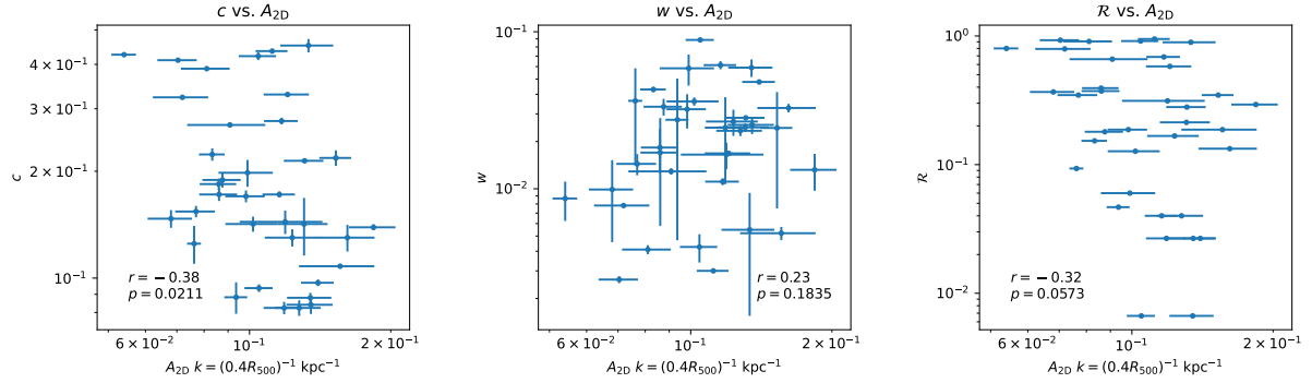
Fig. 4. Morphological parameters c (left), w (middle), and relaxation score \mathcal{R} (right) vs. A_{2D} . The Pearson correlation coefficient and the corresponding p -value are labeled in each panel.
