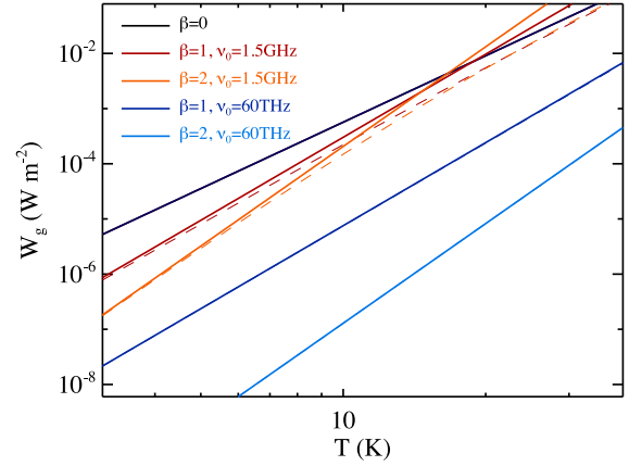
Figure 3. Power radiated by an optically thin greybody versus temperature, for different choices of \beta and v_0 . The black solid line corresponds to the blackbody case ( \beta = 0 ), while red solid lines correspond to v_0 = 1.5 GHz (i.e. \lambda_0 = 200 \mu\text{m} ; dark red: \beta = 1 ; light red: \beta = 2 ) and blue solid lines correspond to v_0 = 60 THz (i.e. \lambda_0 = 5 \mu\text{m} ; dark blue: \beta = 1 ; light blue: \beta = 2 ). Dashed lines represent the optically thick greybody (equation 1): the same colour corresponds to the same parameter combination reported above. Note that for v_0 = 60 THz the two regimes turn out to be indistinguishable in the temperature range shown here, so that dashed lines are completely superposed on the solid lines, then invisible the point where the power of the greybody intersects the power of the blackbody marks the temperature above which the condition of optically thin medium is violated and equation (31) is no longer valid. A colour version of this version is available in the electronic version of the paper.
