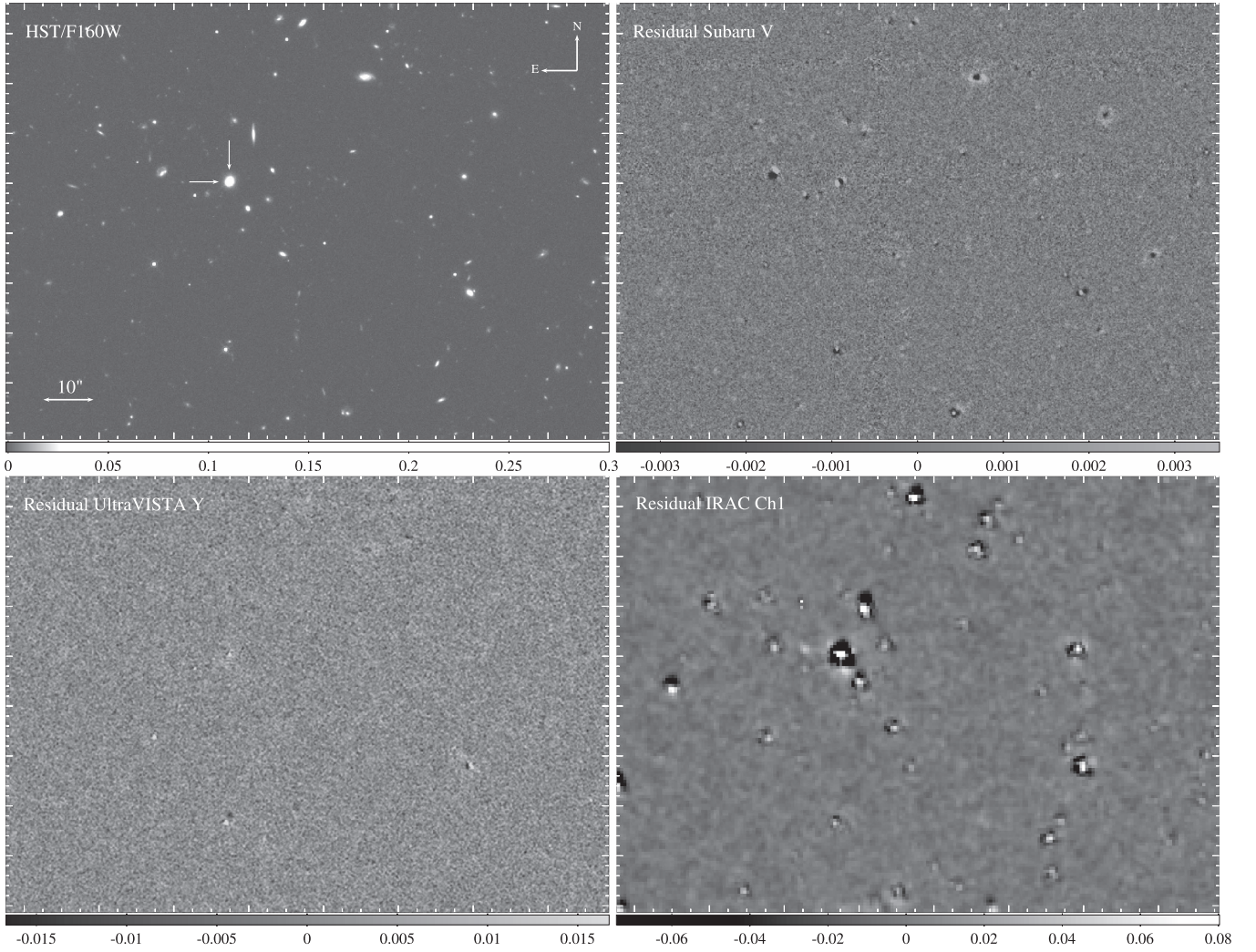
Figure 5. WFC3 F160W source selection band (top left) along with TFIT residual maps in the optical (top right), near-infrared (bottom left) and IRAC infrared (bottom right). The maps all show the same area as the WFC3 F160W band, are in \mu\text{Jy}/\text{pixel} units, and are all scaled linearly as shown by the respective color bars. The background noise for the Subaru V , UltraVISTA Y, and IRAC 3.6\ \mu\text{m} are at the levels of 0.001\ \mu\text{Jy} , 0.004\ \mu\text{Jy} , and 0.006\ \mu\text{Jy} , respectively (images are background subtracted as discussed in Section 3). The arrow marked on the WFC3 maps shows a reference object at a flux density of 74\ \mu\text{Jy} .
