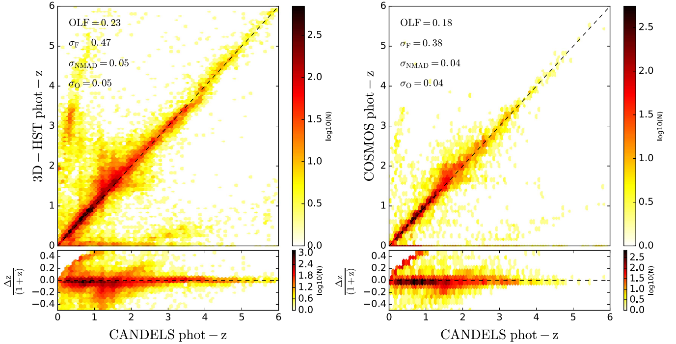
Figure 13. Photometric redshift comparison plots of CANDELS COSMOS with 3D- HST (left) and COSMOS (right) catalogs. The comparison is shown in the form of a 2D histogram with logarithmic bins to help see the small outlier fraction. The sub-panels in both plots show \Delta z / (1 + z_{\text{CANDELS}}) as a function of CANDELS photometric redshifts, where \Delta z = (z_{\text{CANDELS}} - z_{\text{other}}) for photometric redshift measurements.
