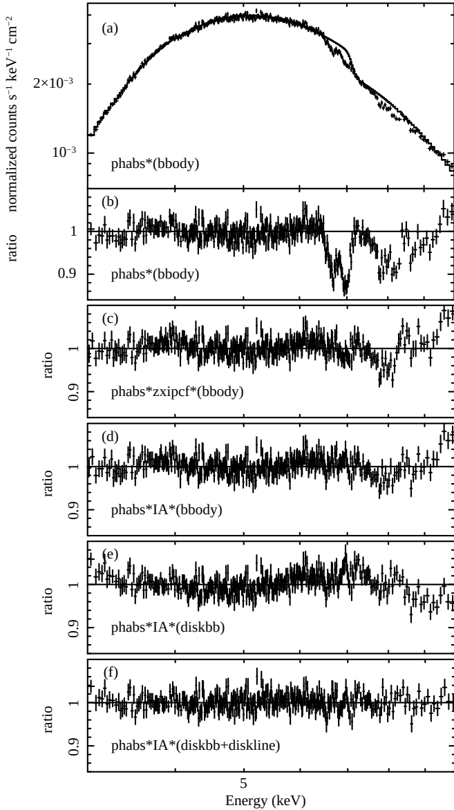
Figure 8. (Panel a): Combined soft state spectra and best-fitting model ( \text{phabs} \times \text{IA} \times (\text{bbody}) ), once the Ionised Absorption (IA) component is removed. (Panel b): Same as panel (a), but showing the data to model ratio. (Panel c): Data to model ratio of the combined soft state spectra with the \text{zxcpcf} component to fit the ionised absorption. (Panels d, e and f): Data to model ratio of the combined soft state spectra with the models: \text{phabs} \times \text{IA} \times (\text{bbody}) , \text{phabs} \times \text{IA} \times (\text{diskbb}) and \text{phabs} \times \text{IA} \times (\text{diskbb} + \text{diskline}) , respectively.
