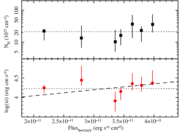
Figure 9. Best fit column density ( N_H , upper panel) and ionisation parameter ( \xi , lower panel) of the photo-ionised plasma, as measured using the \text{zxcpcf} spectral model, as a function of the observed 8–10 keV flux. No significant variation is observed in either of the two parameters (the dotted lines show a model with constant N_H and \xi ). The dashed line shows the best-fitting linear relation between ionisation parameter and source luminosity.
