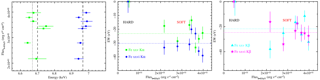
Figure 6. ( Left panel ) Best-fitting energies of the Fe XXV and Fe XXVI K \alpha lines. The vertical lines indicate the energies of the resonance Fe XXVI and Fe XXV lines (dashed) and the inter-combination Fe XXV transition (dotted). ( Middle panel ) Equivalent widths of the Fe XXV and Fe XXVI K \alpha absorption lines (shown in green and blue, respectively) as a function of the 8–10 keV flux. Both lines are significantly detected in each soft state observations, and stringent upper limits can be placed on the lines during the hard state observation. ( Right panel ) Equivalent widths of the Fe XXV and Fe XXVI K \beta absorption lines (shown in cyan and magenta, respectively) as a function of the 8–10 keV flux. In all three panels the error bars indicate the one sigma uncertainties (or limits).
