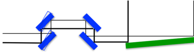
Figure 3: Optical layout of the monochromator (blue) and the beam expander (green). The crystal for monochromation are symmetrically cut, the one for the beam expander is asymmetrically cut. Monochromation with four diffractions, with a possible rigid rotation of the first pair of crystals to detune the rocking curves and so shrink the passing band.
