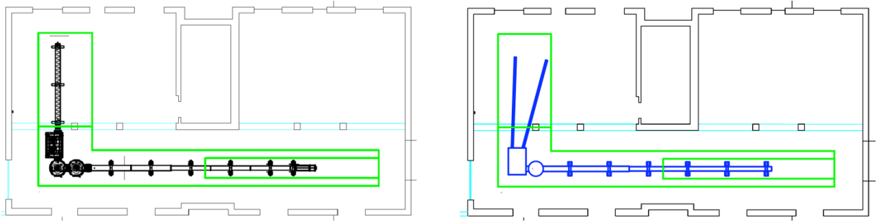
Figure 7: Left: previous design of the BEaTriX 1.0 facility. Right: present design of BEaTriX 2.0.
