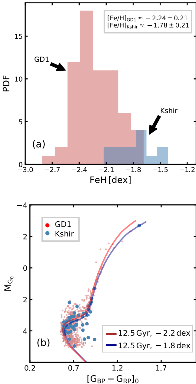
Figure 2. Metallicity and photometry of GD-1 and Kshir. Top panel: [Fe/H] distribution of spectroscopically confirmed members of GD-1 (red) and Kshir (blue) stars. Bottom panel: Gaia (de-reddened) color-magnitude diagram of all member stars of Kshir and GD-1, previously shown in Figure 1. The absolute magnitude was then obtained by correcting the observed magnitude value for the orbital distance of each star. Two SSP template models, corresponding to the mean metallicity values of the streams, are also shown.
