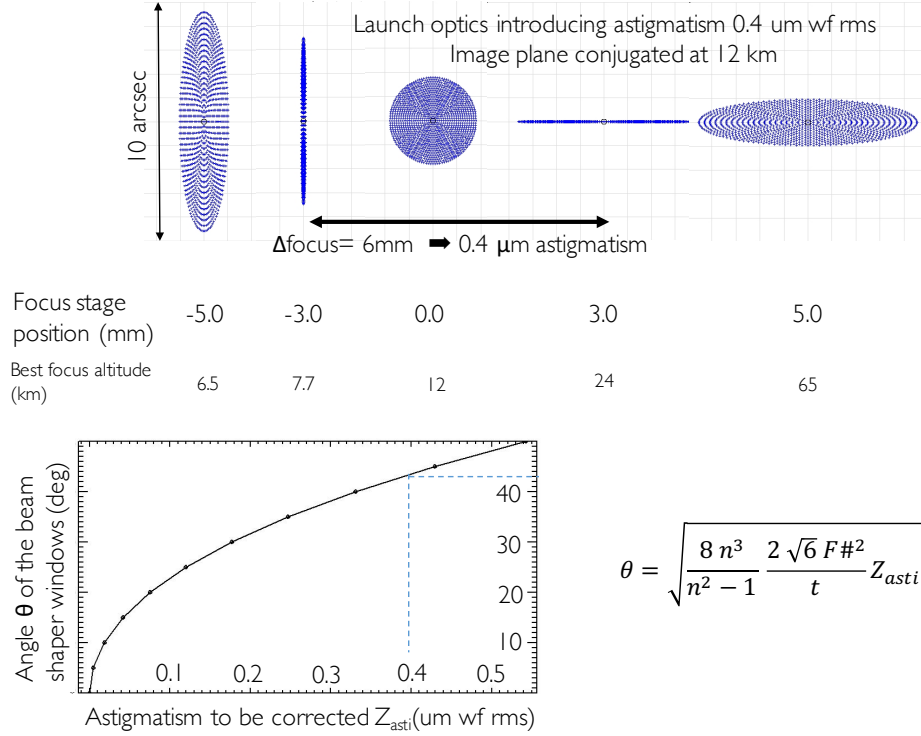
Figure 4. Measurement of a simulated astigmatism in the launch telescope. On top, the images of the launch beam as they would be registered by a device conjugated at 12km while the focus stage range is scanned in 5 steps. The procedure determines the 2 values of the focus stage that minimize the spot size along x and y direction (-3 and 3mm respectively). The difference \Delta focus (6mm in the example) is linearly related to the wavefront astigmatism. The relation has been calibrated using the launch telescope optical model: \Delta focus = 1mm when the beam astigmatism is 70nm rms. Once the astigmatism to be corrected is known, the required angle of incidence on the parallel plate windows of the beam shaping device can be computed according to the relation 20 shown in the bottom of the picture that relates the angle of incidence \theta on the 2 windows of the beam-shaping device with the astigmatism Z_{asti} introduced by the device. t is the window thickness, n the refractive index and F\# the f-number of the beam.
