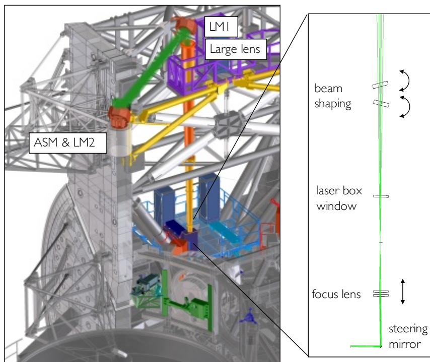
Figure 3. Inside the laser box, the 3 laser beams are recombined over a fast steering pupil mirror used to steer the asterism on sky and for vibration compensation 10 that folds the beams upward. The refractive launch optics consists of 2 positive lenses. The first doublet lens is mounted on a motorized linear stage to adjust focus. The beam shaping device made of 2 counter-tilting parallel plates is installed in the diverging beam after the focus. After about 10m of free path, the beams encounter the second lens of the refractive launch telescope, a large flat mirror LM1 and a second large mirror LM2 installed on the back of the ASM that projects the 3 beams on sky. The LM1 is motorized for a coarse, wide range adjustment of the laser pointing.
