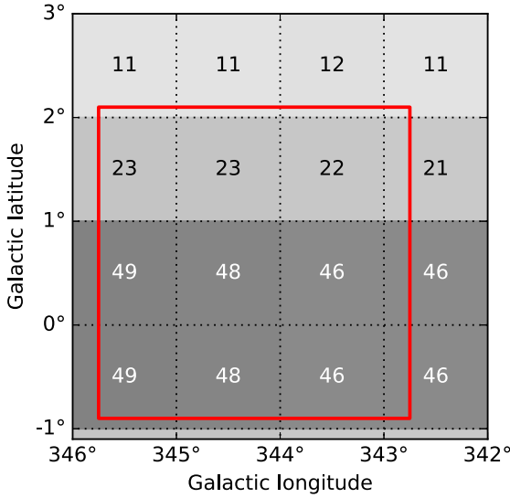
Figure 5. Number of PNe per square degree towards the SCORPIO region (delimited by the thick line), assuming a total number of 20 000 Galactic PNe and an exponential distribution.
