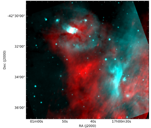
Figure 9. Two-colour image of the known H II region SCO J170049–423153 (in red our radio data, in cyan GLIMPSE at 8\ \mu\text{m} ). This is an example of a diffuse radio source which is a known H II regions and can be used as a prototype for this kind of objects.
