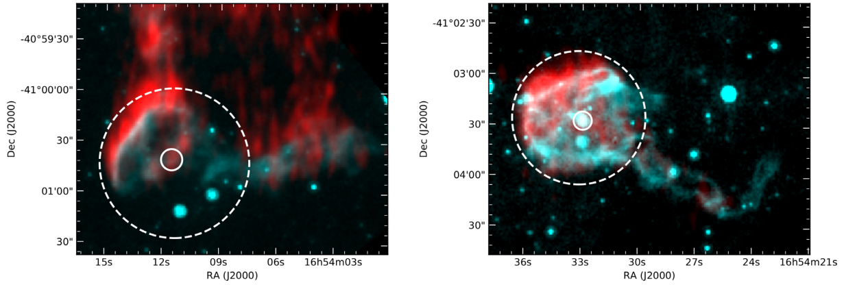
Figure 7. Two-colour images of the LBV/WR star candidates SCO J165412–410032 (left) and SCO J165433–410319 (right; in red our radio data, in cyan GLIMPSE at 8 \mu m). The dashed circle highlights the external shell, while the solid circle the central object.
