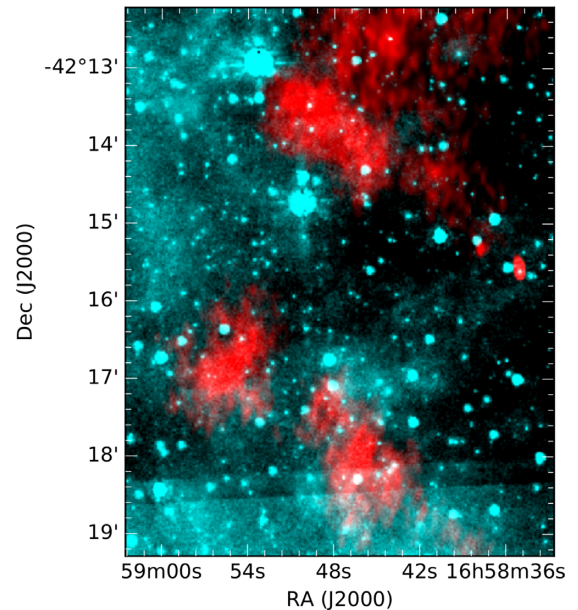
Figure 10. Two-colour image of the extended sources SCO J165843–421308, SCO J165844–421814, and SCO J165855–421638 (in red our radio data, in cyan GLIMPSE at 8\ \mu\text{m} ). All these three sources are new detection, and we classified them as diffuse sources. While the top sources has an anticorrelating counterpart in the IR, the bottom ones do not.
