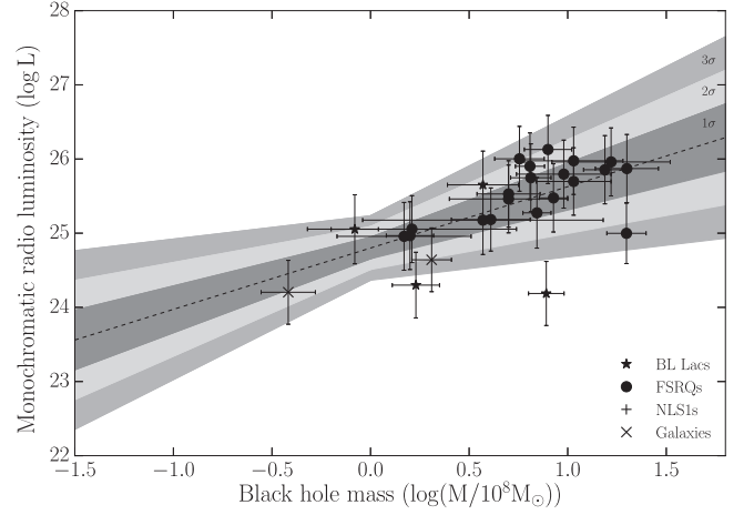
Figure 2. Intrinsic monochromatic radio luminosity (4.8 GHz) vs. M_{\text{BH}} . The dashed line indicates the best-fit model. Symbols and gray areas are the same as in Figure 1.
