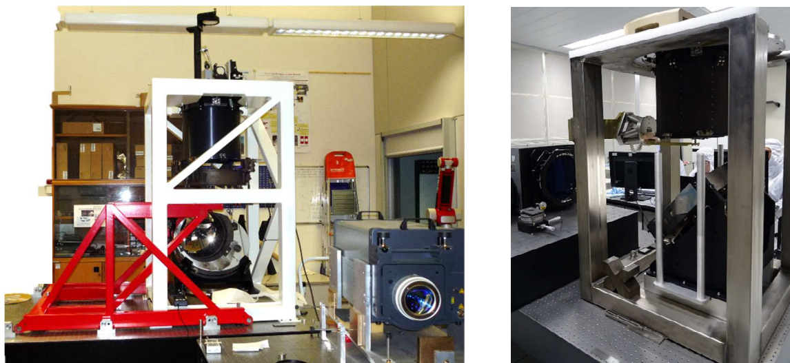
Figure 3: Left : DM M2 alignment setup. Right : PFM M2 alignment setup. In both cases is visible the Zygo interferometer feeding light to the tube thanks to a 45^\circ oriented large flat mirror. The tube is held in vertical configuration, M2 is adjusted thanks to a manipulator fixed to the red handling on DM and to a hexapod or PFM. Also, the reference flat mirror located over OBA can be seen in both cases.
