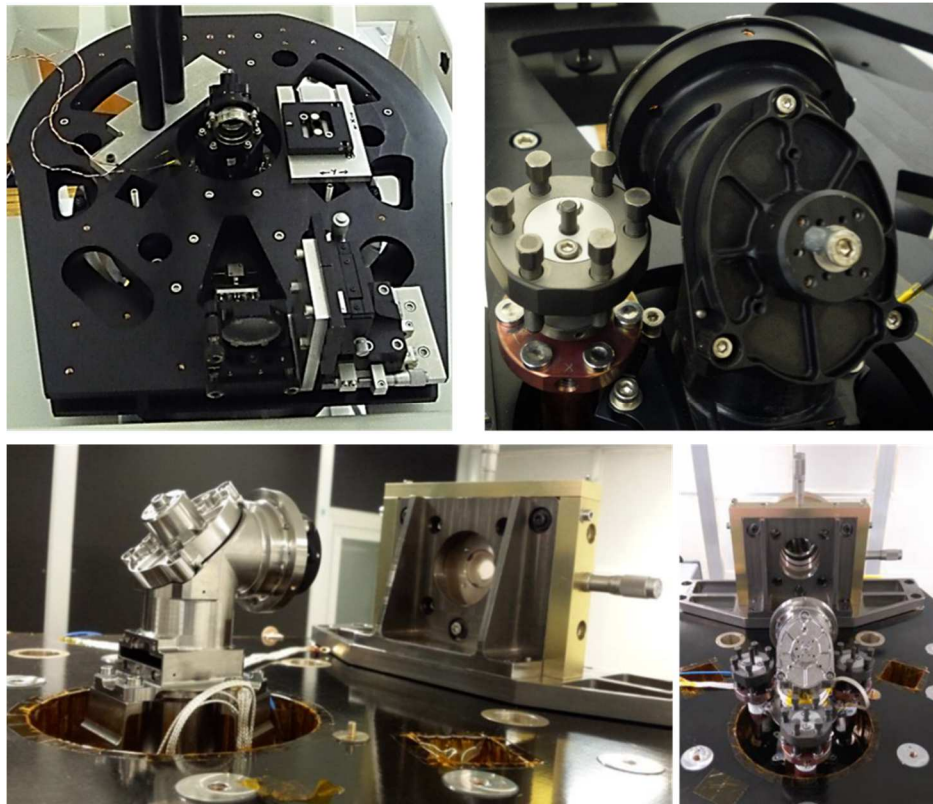
Figure 4: Top panels : DM BEO alignment. One pre-tensioning tool was used. Bottom panels : PFM BEO alignment setup. Three pre-tensioning tool were used as lessons learned from DM activities.
