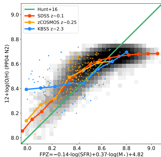
Fig. 1. So-called fundamental plane by Hunt et al. (2016), as derived by PCA of a sample of \sim 1000 low metallicity starbursts, shown as a green line. The distribution of SDSS galaxies from M10 is overplotted with their median metallicity values in mass bins shown in red. The high- z samples with a significant number of galaxies and z < 3 and measured N2 index used by Hunt et al. (2016) are also reported; the zCOSMOS galaxies at z \sim 0.25 from Cresci et al. (2012) are indicated in orange and the KBSS z \sim 2.3 galaxies from Steidel et al. (2014) in blue. All metallicities have been derived with the same calibration based on N2 (Pettini & Pagel 2004). Small dots represent the single galaxy measurements, while the larger circles the medians in mass bins. The general population of local star-forming galaxies, as traced by SDSS, as well as the higher z samples are not well reproduced by the plane.
