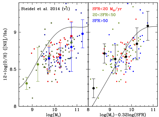
Fig. 7. MZ and FMR relation for the Steidel et al. (2014) sample. In the left panel the MZ relation is shown; galaxies are colour coded into three bins based on their measured SFR. The black solid line shows the z=0 M10 MZ relation using SDSS galaxies; the observed offset from the z \sim 2 galaxies is due to the evolution of the MZ relation. The error bars represent the 1\sigma dispersion in each bin. The right panel shows the FMR \mu_{0.32} projection for the same data points; the black points indicate medians in bins of \mu_{0.32} , showing that the Steidel et al. (2014) z \sim 2.3 sample is reasonably reproduced by the FMR defined with SDSS galaxies at z=0 (shown in black).
