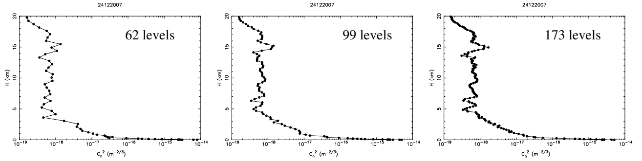
Figure 62: Vertical profiles of the average simulated C_N^2 with different vertical resolutions, for a night in 2007. Left: with 62 levels; Middle: with 99 levels; Right: with 173 levels.
