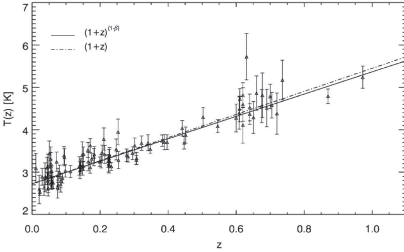
Fig. 2. Measurements of the CMB temperature as a function of redshift for 104 Planck selected clusters. The solid line is the best fit to the scaling T_{\text{CMB}}(z) = T_{\text{CMB}}(0)(1+z)^{1-\beta} . The dot-dashed line is the standard scaling, with \beta = 0 . Picture taken by Luzzi et al. 70 see there for details (courtesy G. Luzzi).
